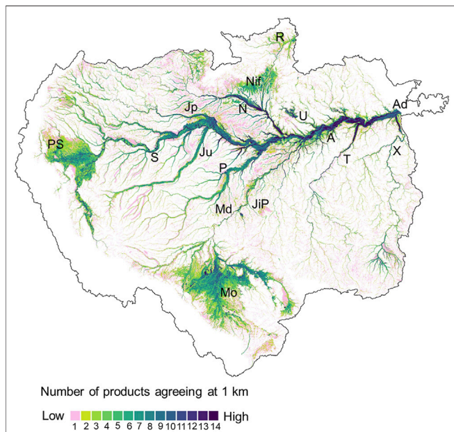
FIGURE 2 | Hydrological Amazon basin with inundated areas shown for basin <500 m asl based on different remote sensing and analysis techniques. Each 1 km pixel shows the number of basin-scale inundation datasets (total of 14 products were assessed) that agree that the pixel is floodable, according to Fleischmann et al. (2021). Rivers and wetlands mentioned in the text: Solimões—S, Madeira—Md, Negro—N, Japurá—Jp, Juruá—Ju, Purus—P, Amazonas—A, Tapajós—T, Xingu—X, Ji-Paraná—JIP, Uatumã—U, Llanos de Moxos - Mo, Pacaya-Samiria - PS, Negro interfluvial wetlands - Nif, Roraima—R, Amazon delta wetlands—Ad.
