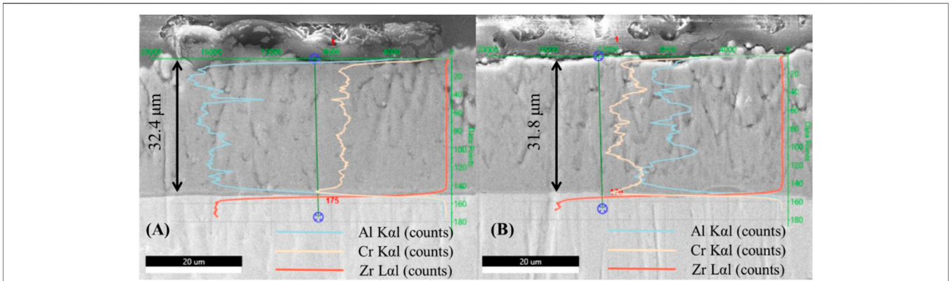
FIGURE 10 | EDS results of cross-section of each ATF candidate cladding with 6 h deposition: (A) Cr_{32.1}Al_{67.9} , (B) Cr_{45.8}Al_{54.2} .
