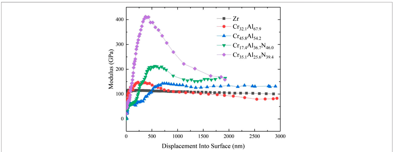
FIGURE 11 | Relationship of Young's modulus-indentation depth for Zr-4 and coatings.
