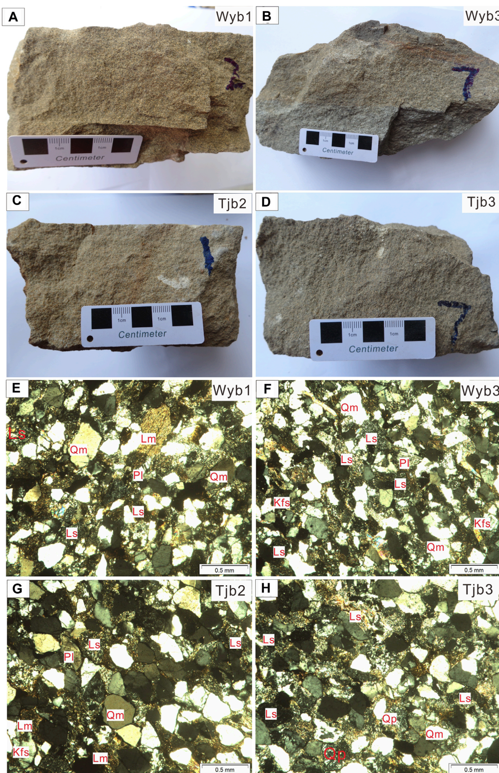
FIGURE 3 (A–D) Hand specimen and (E–H) microscopic photos of sandstone samples from the WSS and TNES. Abbreviations: Qm-monocrystalline quartz; Qp-polycrystalline quartz; Pl-plagioclase; Kfs-K-feldspar; Ls-lithic fragments of sedimentary rocks; Lm-lithic fragments of metamorphic rocks; Lv-lithic fragments of volcanic rocks.
