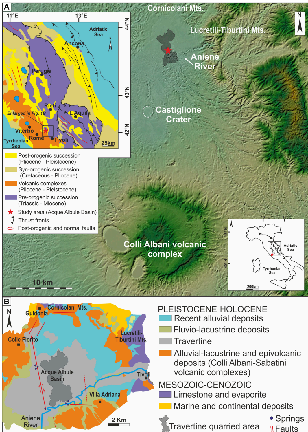
FIGURE 1 (A) Geological map of Central Italy with an indication of the study area (square) and a digital elevation model of the study area (modified from Tarquini et al., 2023). (B) Geological map of the Acque Albule Basin (modified from Mancini et al., 2021).
