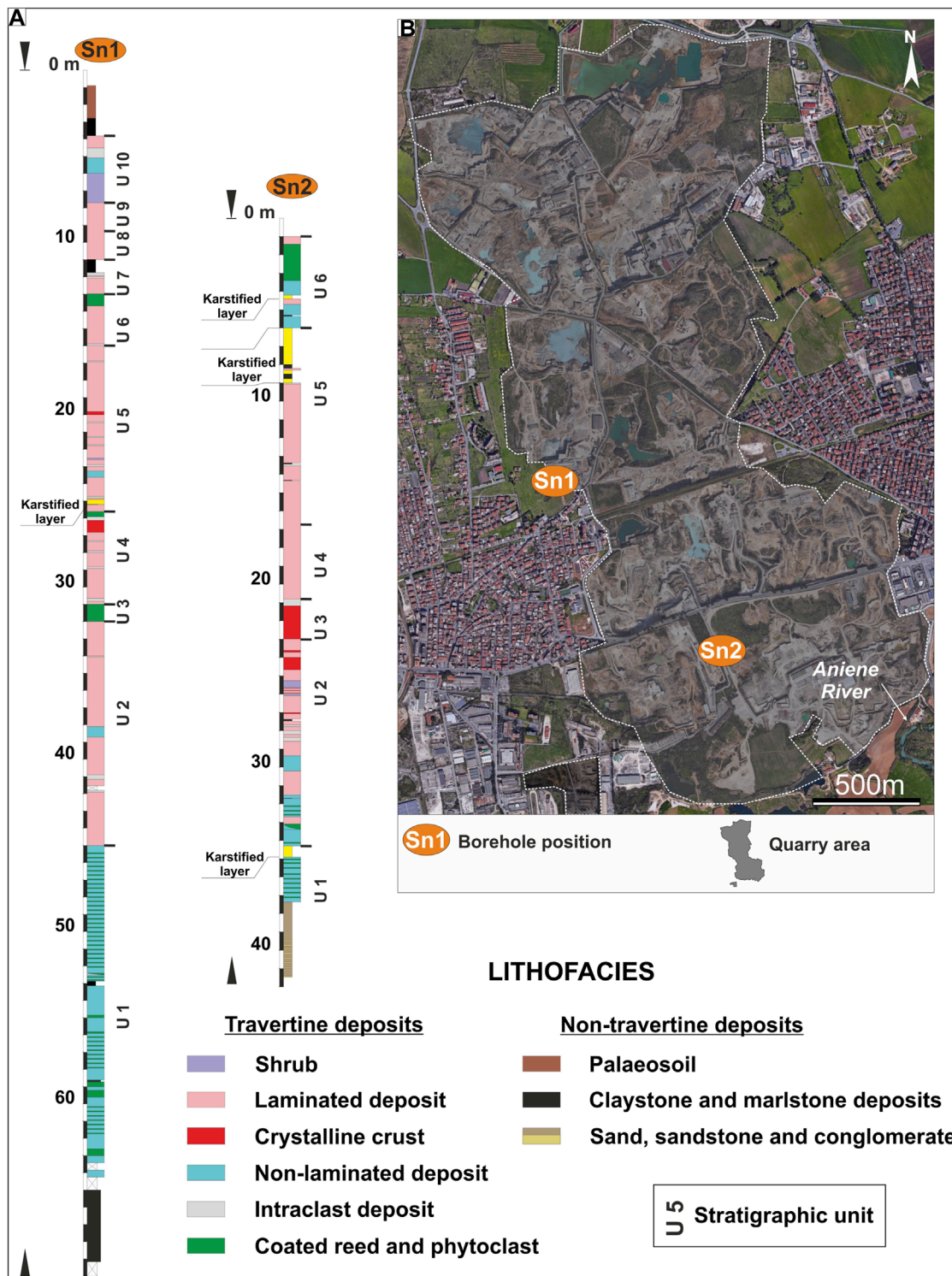
FIGURE 2 (A) Stratigraphic log and pictures of Sn1 and Sn2 boreholes showing the lithofacies, divided in travertine and non-travertine deposits, and depositional units; (B) map showing positions of Sn1 and Sn2 boreholes (modified from Google Earth, 2023).
