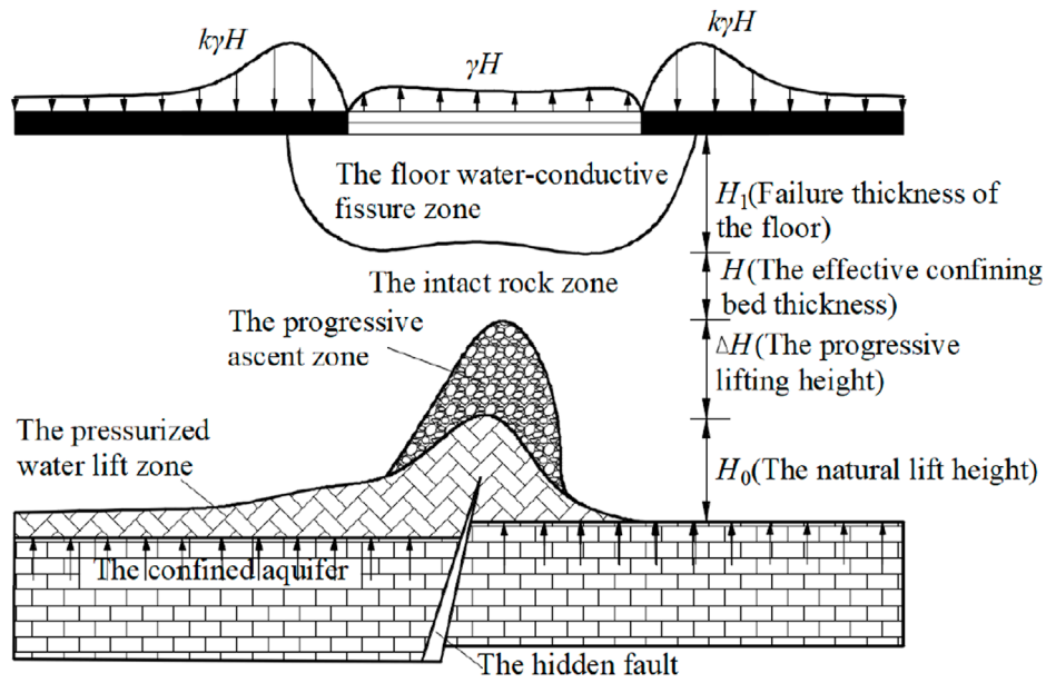
FIGURE 8 Progressive ascending principle and segregation diagram of coal layer seam (Wang et al., 2018a; Wang and Yao, 2022)
