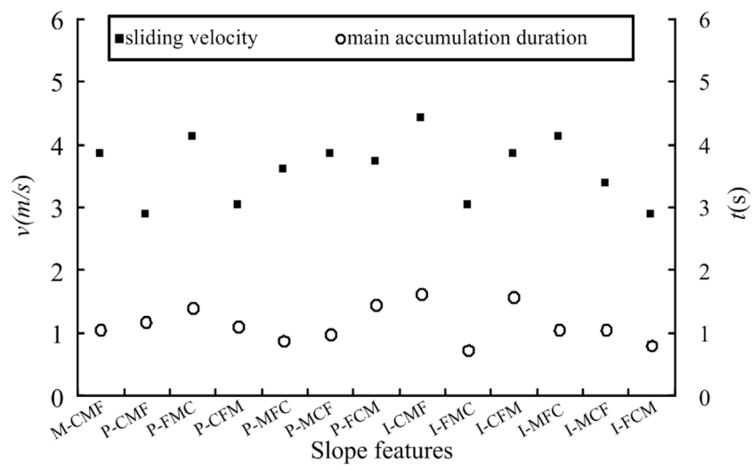
FIGURE 11 Average velocity and accumulation stage duration of a landslide under different slope conditions.
