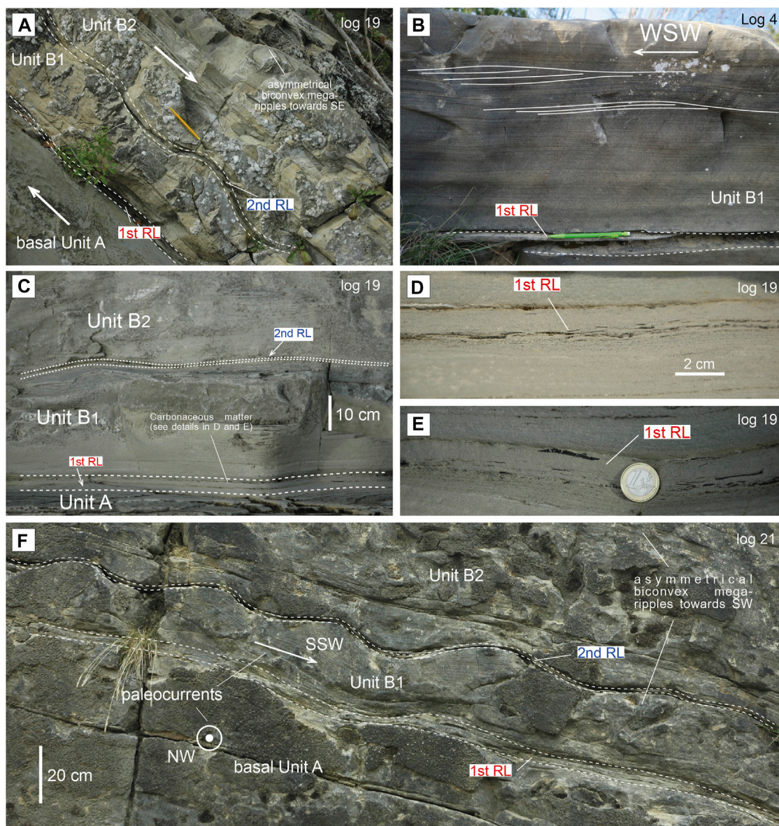
FIGURE 5 | (A) Examples of facies B1 and B2 in Log 19 (Santerno valley) separated by the 1 st (red) and 2 nd (blue) evident rebound layers; (B) Facies B1 in Log 4 (Lamolli) with evidence of lateral deflections; (C) Facies B1 and B2 separated by the 1 st (red) and 2 nd (blue) rebound layers in Log 19; (D,E) First rebound layer separating facies A and B rich in carbonaceous matter (see C for the location of the photos); (F) Facies B1 and B2 separated by the 1 st (red) and 2 nd (blue) rebound layers (Log 21); to be noted the slightly asymmetrical megaripples with paleocurrents towards the SW in Unit B1 (see Figure 4 for the location of the Logs).
