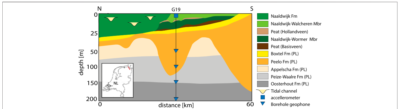
FIGURE 1 | Schematic geological cross section of the upper 200 m of the soft sedimentary cover in the northeastern Groningen region (red line in inset). Note that the vertical scale is inflated for the top 50 m to highlight the stratigraphy of the Holocene formations on top of the Pleistocene (PL) formations. Borehole station G19 is featured because this site is used for wave-propagation modeling. The G-network vertical arrays consists 5 seismometers (accelerometer (blue square) at the surface and geophones (blue triangles) at depth) with a 50 m depth interval. This cross section is based on GeoTOP ( www.dinoloket.nl ).
