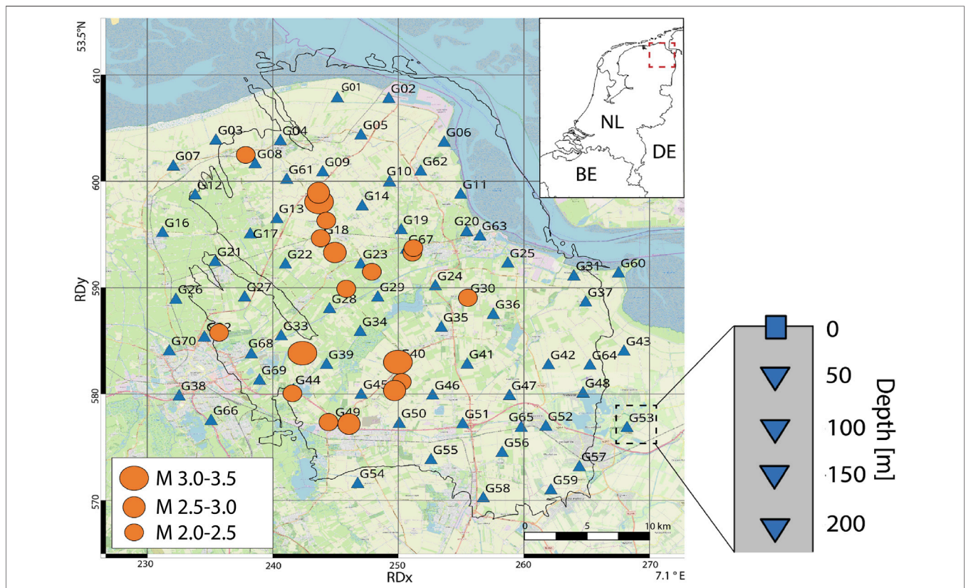
FIGURE 2 | Map view of the Groningen borehole network in the northeast of the Netherlands. The triangles represent the surface location of each borehole site in the network. Each borehole contains an accelerometer at the surface and four 4.5 Hz geophones at depth with a 50 m depth spacing. The orange circles represent the local earthquakes with magnitude 2 or higher, recorded in the G-network between 05–2015 and 05–2019. Coordinates are shown within the Dutch National Triangulation Grid (Rijksdriehoekstelsel or RD) and lat/lon coordinates in the corners for international referencing. Background map: OpenStreetMap contributors, CC-BY-SA, www.openstreetmap.org .
