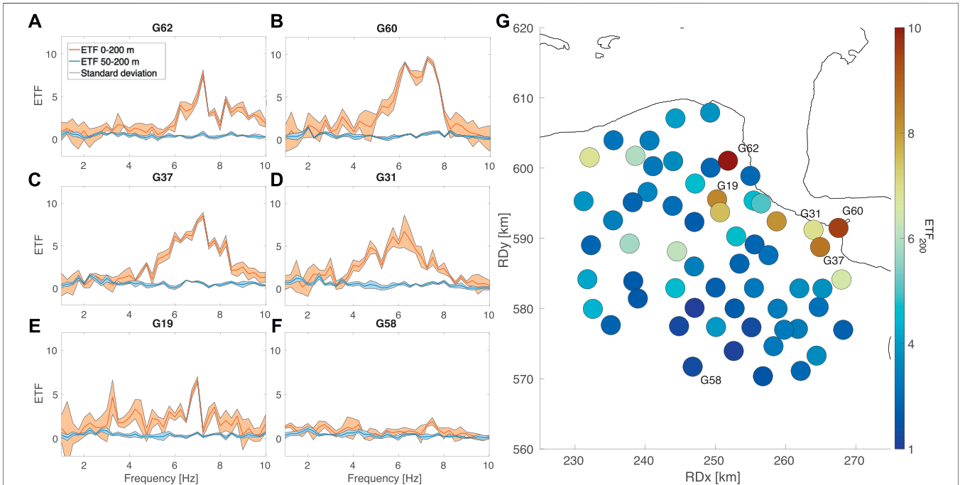
FIGURE 7 | (A) Each panel depicts the empirical transfer functions (ETFs) between the seismometer at 200 m depth and the surface (red) and standard deviation (pale red area) for sites G19, G31, G37, G60, and G62, displaying the frequency-dependent amplification. The blue lines illustrate the ETFs between the seismometers at 200 m and 50 m. Borehole G62 additionally depicts the ETF between the surface and 50 m seismometer (gray). Borehole G58 is added as example of a borehole site with no amplification measured. (B) Spatial distribution of the peak amplitudes from the ETF for 60 borehole station sites.
