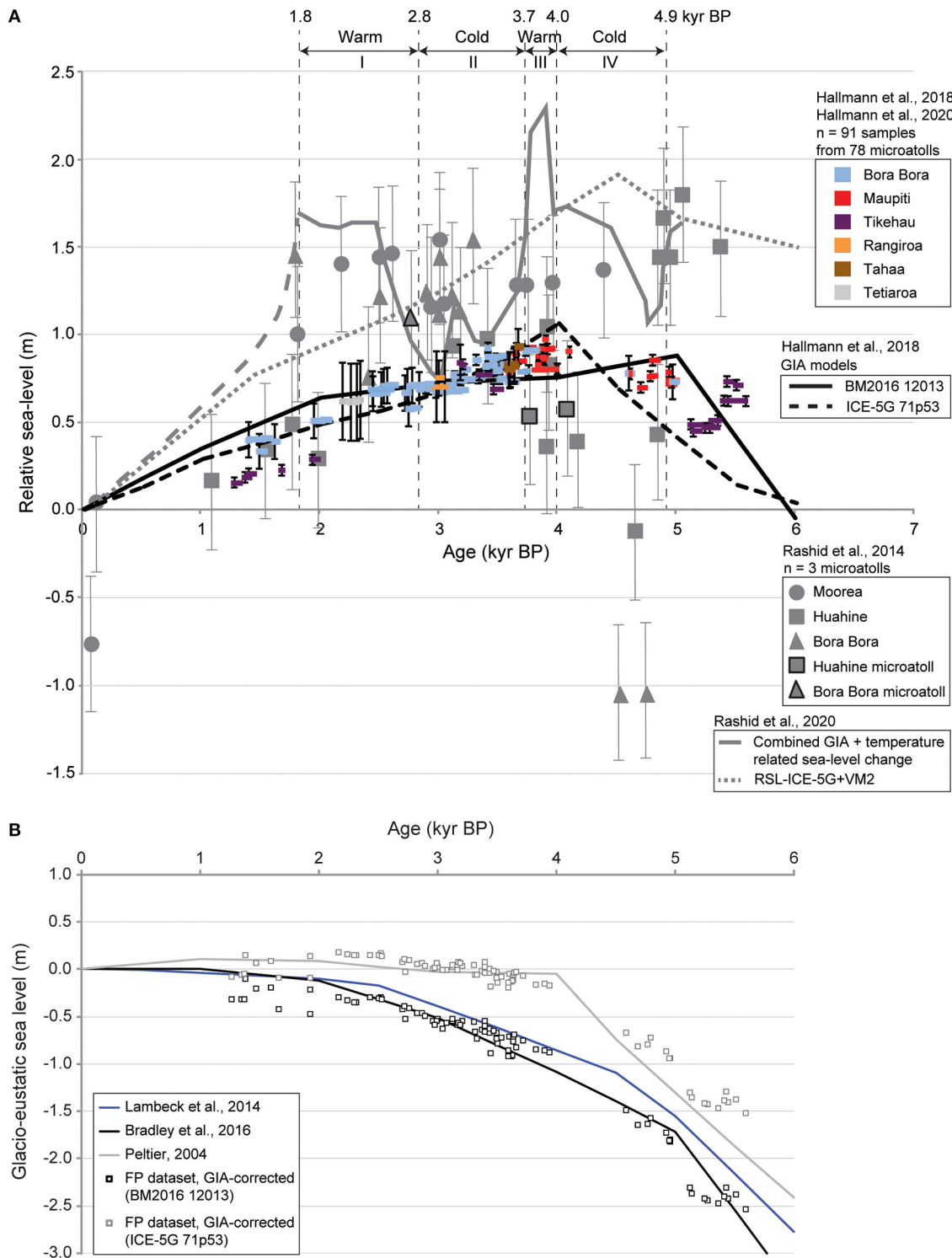
FIGURE 1 | (A) Reconstructed mid- to late-Holocene RSL changes in French Polynesia (Hallmann et al., 2018, 2020; in color) compared to model outputs based on BM2016 (black solid line) and ICE-5G ice models (black dashed line). This reconstruction overlies sea-level estimates from Rashid et al. (2014; in gray), their ICE-5G model output (gray dashed line) and the combined GIA-temperature related sea-level change presented in Rashid et al. (2020; gray solid line). For the Hallmann et al. (2018, 2020) dataset, the BM2016 model captures the older data better than ICE-5G as it produces an earlier highstand, however, the curve produced by ICE-5G better tracks the observations for the period after 4 kyr BP. This is also reflected in the consistency between the model curves (black and gray lines) and the model-corrected data (black and gray boxes) in (B) . In contrast to the 1-m sea-level highstand revealed by Hallmann et al. (2018, 2020), the ICE-5G model by Rashid et al. (2014) results in a ~2-m sea-level highstand. However, the Rashid et al. (2014) dataset is scattered and only one microatoll from Bora Bora is consistent with the (Continued)
