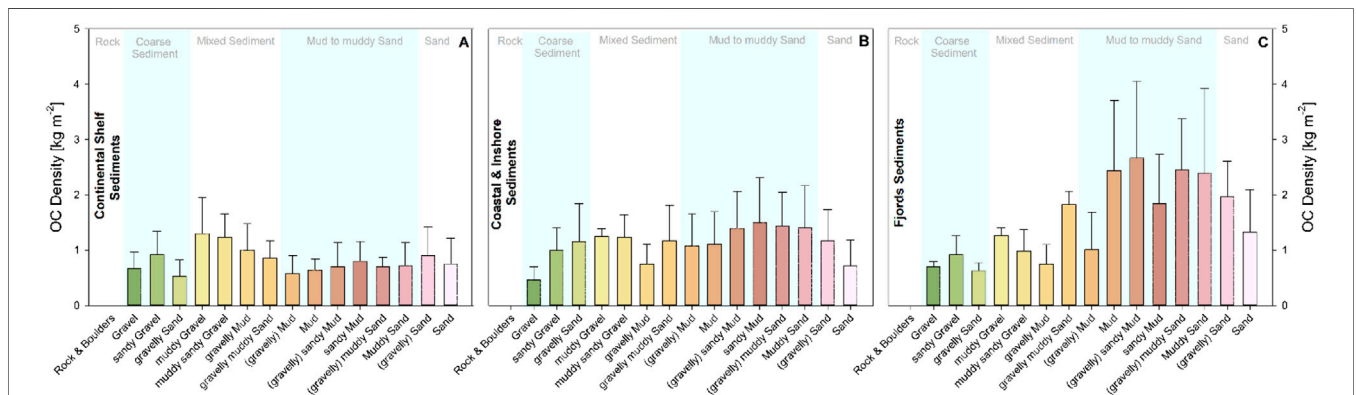
FIGURE 8 | Mean OC density [ \text{kg m}^{-2} ] of the 16 sediment classes across the three UK EEZ zones (A) Continental shelf (and shelf slope and deep sea zone) (B) Coastal and inshore (C) Fjords.
