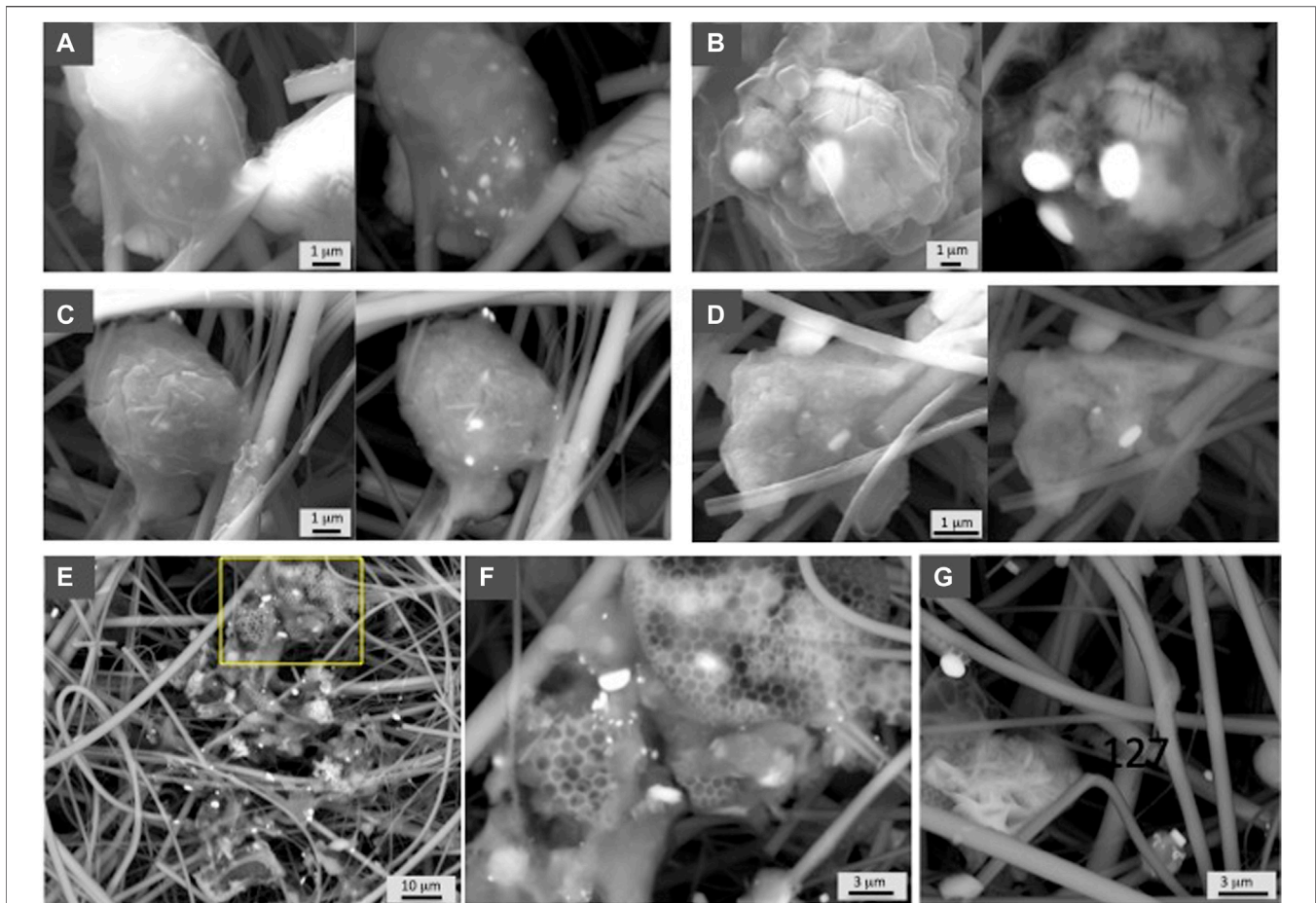
FIGURE 3 | SEM photographs showing representative examples of barite from the Atlantic sector analyzed in this study. Samples are indicated in Table 1 . Both secondary electron and in backscattered electron (BSE) mode at 30 kV are shown in each sample. (A) GCM 122 (112 m), (B) GCM 123 (162 m), (C) GCM 124 (300 m), and (D) GCM 126 (750 m). (E) GCM 125 (500 m) shows the barite abundance at 500 m depth, and (F) GCM 127 (1,000 m) shows a detailed image of the square indicated in photograph e, in which different sizes of barite grains are shown in organic aggregates. (G) GCM 127 corresponds to the deepest filter sample obtained at this ocean sector, 1,000 m, in which barite is not abundant but still present.
