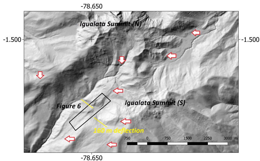
FIGURE 5 | Zoom-in of the Igualata center area. The figure highlights several sharp scarps and deflecting lineaments across the covered area, along the red arrows. The figure focuses on the lineament that includes the Figure 6 features and that seems to cause the 160 m right lateral deflection of the major incision (underlined in yellow).
