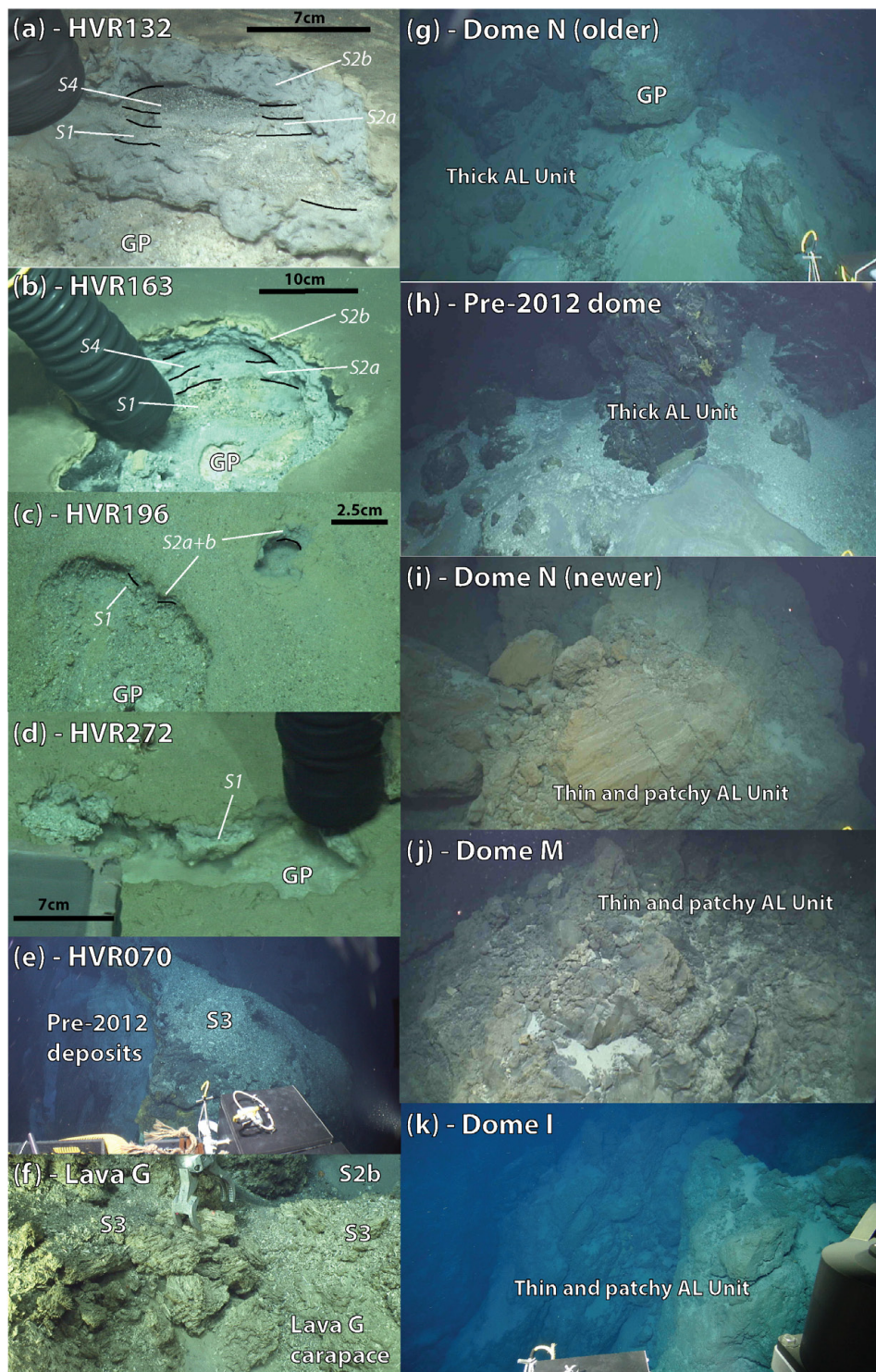
FIGURE 2 | Seafloor images of AL unit layering exposed during sampling from atop GPs at locations HVR132 (a) , HVR163 (b) , HVR196 (c) , and HVR272 (d) . At both HVR132 (a) and HVR163 (b) a similar stratigraphy can be observed showing four layers with comparable layer thicknesses, apparent grainsize, and color. At HVR196 (c) only two layers can be seen. At HVR272 (d) only a single layer can be seen (e and f) show a clastic deposit consisting of lapilli and ash with dominantly elongate tube morphologies at HVR070 (e) and overlying the carapace of Lava G (f) . In (g-k) , the variation in the AL unit coverage overlying lavas around the caldera is shown. Thick deposits of the AL unit can be seen overlying an apparently older part of Lava N (g) and also overlying a lava produced prior to the 2012 Havre eruption (h) . Over the more-recent part of Dome N (i) , and on Domes M (j) , and I (k) , the AL unit is thinner and patchier. Domes with similar shapes were chosen to provide a consistent context for observed variations in the AL unit.
