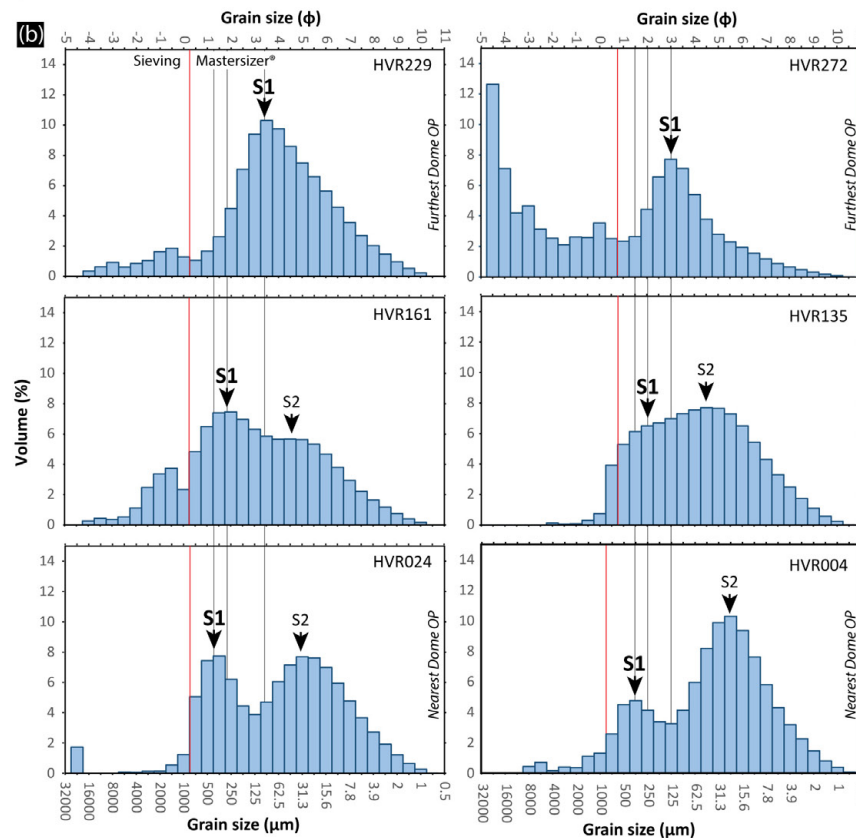
FIGURE 4 | (a) Sample numbers and grainsize peaks for samples of the AL unit from 0.25 \phi (~240 \mu\text{m} ) and 3.5 \phi (~88 \mu\text{m} ), inferred to represent S1, across the Havre caldera. (b) Representative grain size distributions for samples of the AL unit, with samples closest to Dome OP at the bottom and samples furthest away at the top. The dark lines show the location of the inferred S1 peak in each sample for comparison across the caldera. Note the lack of the 5–6 \phi mode on the northern caldera rim in samples HVR229 and HVR272.
