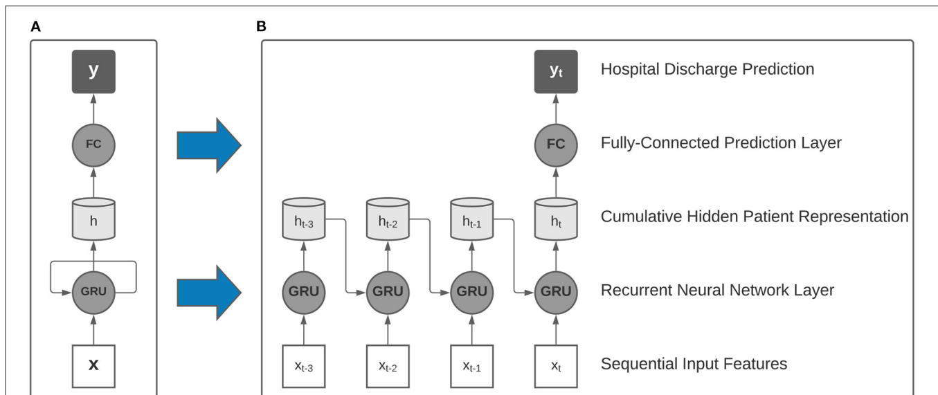
FIGURE 2 | Collapsed (A) and expanded (B) view of a single-layer recurrent neural network with gated recurrent units (GRU) used as building blocks in our model. After processing multi-resolution sequences of vital signs and activity sensor data, a final hospital discharge prediction was made using the final hidden representation.
