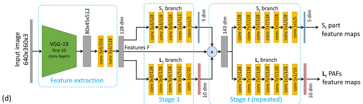
FIGURE 3 | Pose detection model. (a) 5 parts skeleton (Head, Thorax, Abdomen, Left and Right Antenna) and connection used. (b) Confidence map of the abdomen keypoints used to train the (S) branch. (c) The magnitude of the Part Affinity Field (PAF) of the thorax-abdomen connection used to train the (L) branch. (d) Convolutional Neural Network architecture used to predict the body part confidence maps and PAFs organized as a feature extraction backbone followed by the two branches (S) and (L) with iterative refinement stages.
