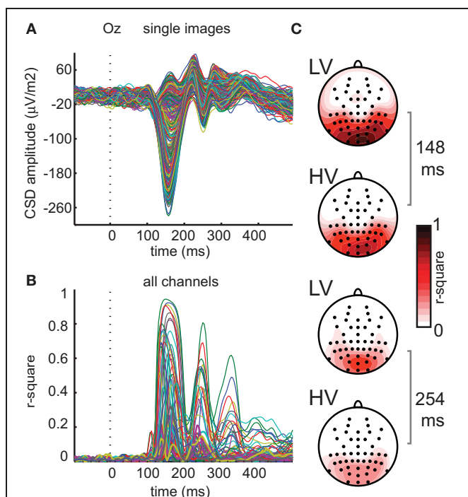
FIGURE 5 | Regression analyses on mean ERP data for all channels. (A) Individual image ERPs converted to current source density signals (CSDs) averaged over subjects at channel Oz. (B) Explained variance at each time-point resulting from regression analyses of mean ERP amplitude on contrast statistics of the 400 texture images (average of two presentations) at all 64 electrodes. (C) Results of regression analysis based on mean ERP for all electrodes, at two time-points of peak explained variance (148 and 254 ms), indicating substantial explained variance on electrodes overlying visual cortex for both high-variant (HV) and low-variant (LV) texture categories.
