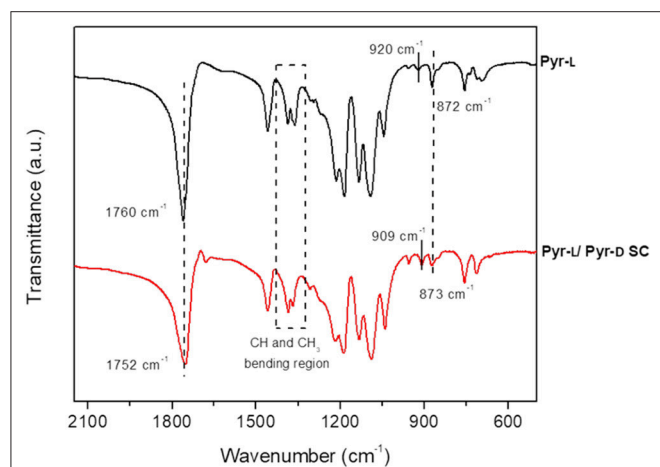
FIGURE 3 | FTIR spectra ( 500 – 2,250\text{ cm}^{-1} region) of Pyr-L (black) and Pyr-L/Pyr-D SC (red) after crystallization in DMF.
