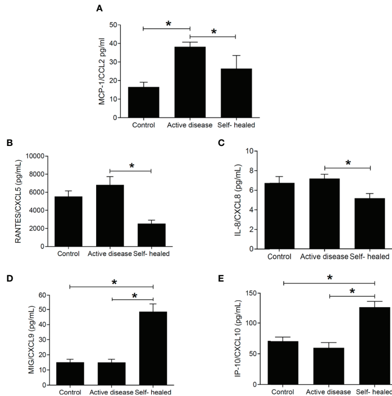
FIGURE 7 | Chemokine concentration (pg/ml) in plasma of cutaneous leishmaniasis patients and controls. MCP1/CCL2 ( A ), RANTES/CXCL5 ( B ), IL-8/CXCL8 ( C ), MIG/CXCL9 ( D ), and IP-10/CXCL10 ( E ) concentrations were measured by flow-cytometry using the CBA kit. * = p < 0.05 (Kruskal-Wallis and Bonferroni tests). N = 5 patients and controls per group.
