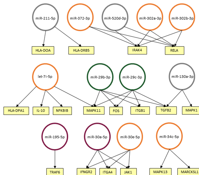
FIGURE 4 | Predicted interactions between the set of differentially expressed microRNAs in THP-1 cells after 6 and 24 h post infection. The genes on which they are suggested to act in the Leishmaniasis pathway in humans are shown as seen in KEGG. miRNAs were classified into four groups according to their modulation through time: down-regulated in 6 and 24 h (A), up-regulated on 6 h and down-regulated in 24 h (B), down-regulated in 6 h and up-regulated in 24 h (C) and up-regulated in both timepoints (D).
