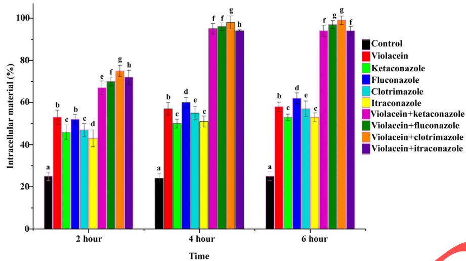
FIGURE 5 | Rate of release of intracellular material of T. rubrum recorded absorbance at 260nm in the absence (control) and presence of violacein/azoles alone and in combination. Data are
