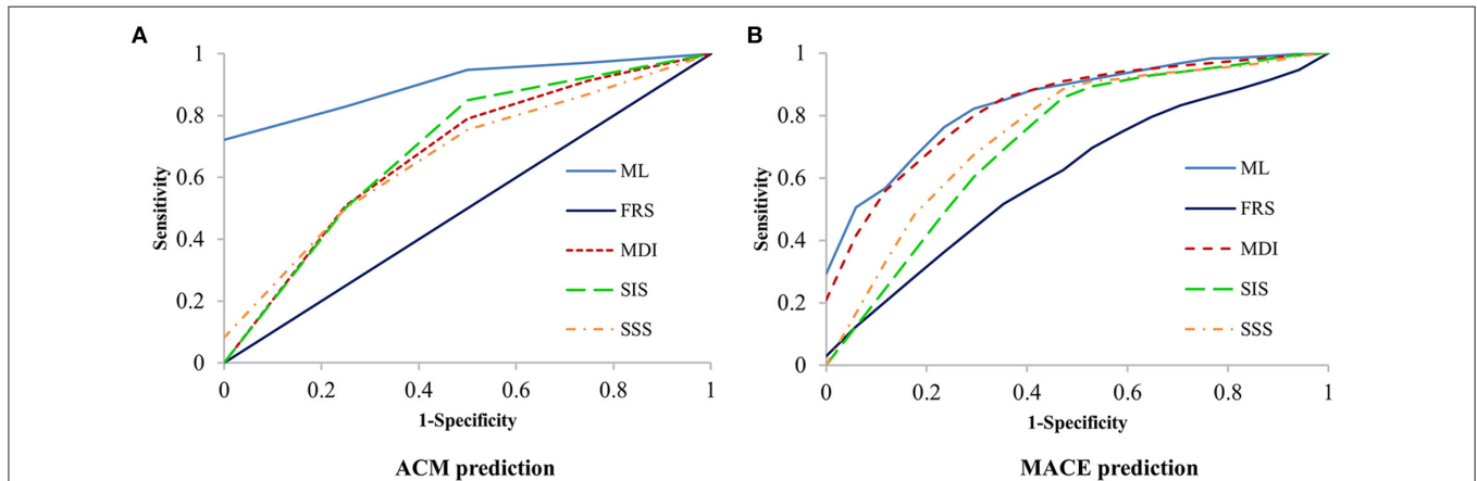
FIGURE 4 | Receiver-operating characteristic (ROC) curves for prediction of ACM and MACE. Machine learning had a significantly higher area-under-the curve for prediction of ACM ( P < 0.001 , A) and MACE ( P < 0.05 , B) than all other scores. ACM, all-cause mortality; FRS, Framingham risk score; MACE, major adverse cardiac events; MDI, modified Duke index; SIS, segment involvement score; SSS, segment stenosis score.
