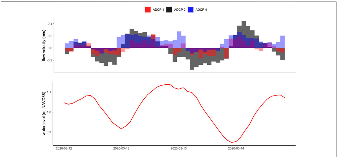
FIGURE 10 | Temporal shifts in the water flow direction at the Redfish Lake inlet (ADCP4) are both delayed and lag behind those at the Carancahua inlet (ADCP2). For several hours of the record, they flow in opposite directions.
