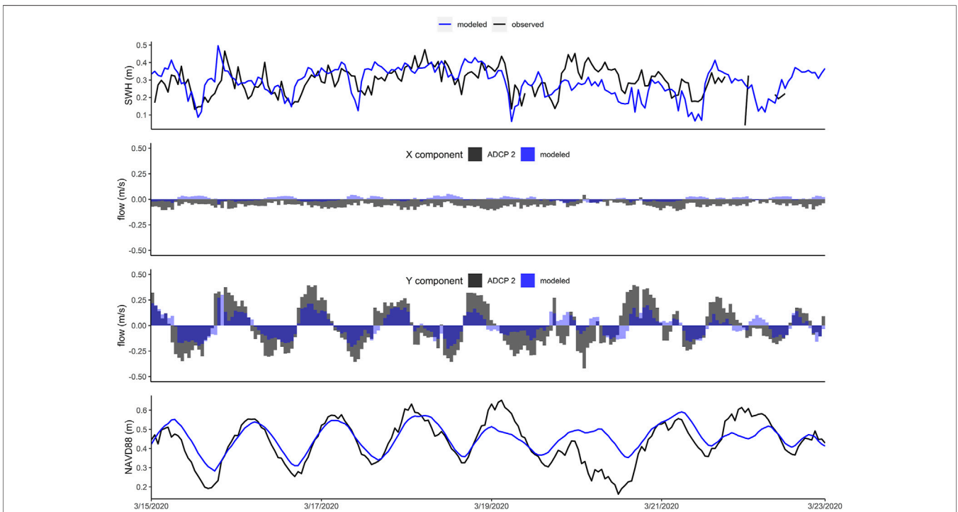
FIGURE 11 | Comparison of measured and modeled hydrodynamics at Carancahua inlet.
