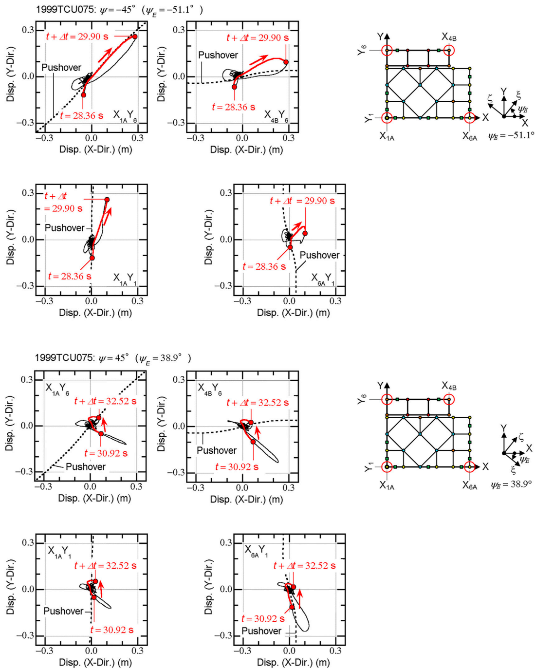
FIGURE 13 Displacement orbit of the four isolates at the corners.
