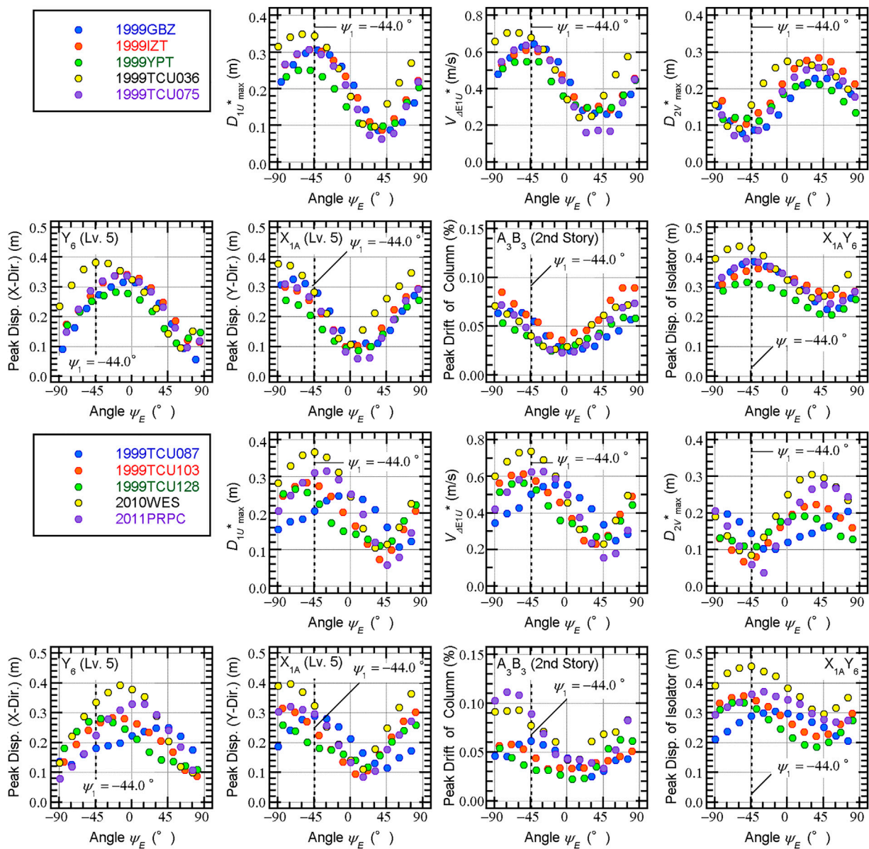
FIGURE 10 Relationship between the peak response and the ASI defined in terms of the principal axis based on the cumulative energy input.
