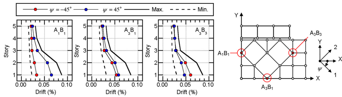
FIGURE 14 Peak drift of the three columns A_1B_1 , A_3B_1 , and A_3B_3 (1999TCU075).
