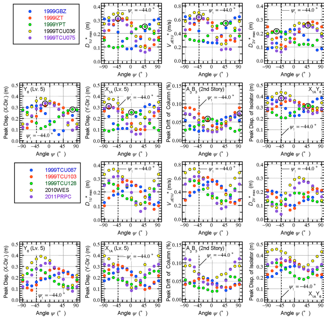
FIGURE 9 Relationship between the peak response and the angle of seismic incidence (ASI) defined in terms of the principal axis of Arias. Note that the plot at -90^\circ is added to consider the symmetry: the plots at -90^\circ and 90^\circ are the same. The black circled plots indicate the largest responses for the 1999YPT and 1999TCU075 cases.
