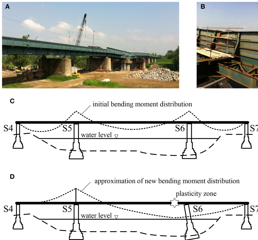
FIGURE 1 | (A) Damaged steel railway bridge; (B) plastic hinge on the upstream girder; (C) bending moment before damage; (D) approximation of bending moment after damage.
