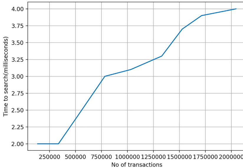
FIGURE 11 | Transaction/asset search performance in the Vind blockchain platform.
