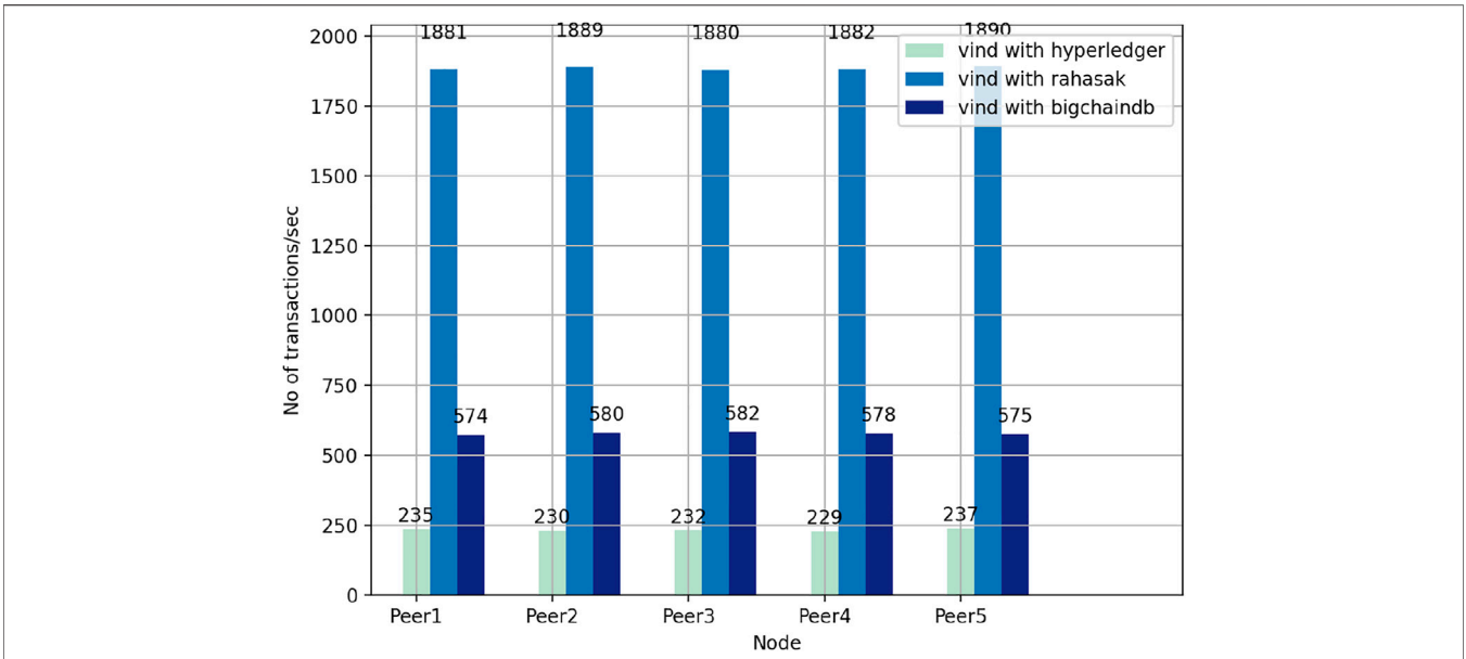
FIGURE 6 | Query transaction result of the Vind platform with different blockchain ledgers.
