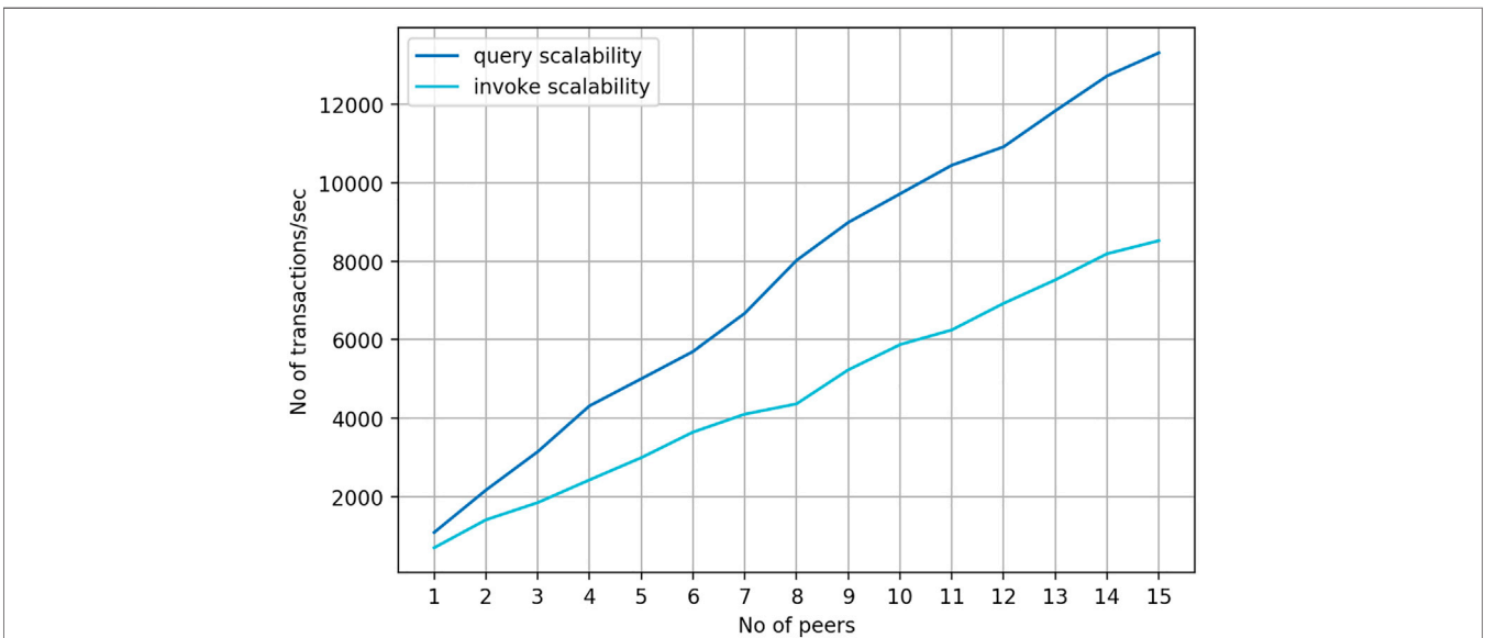
FIGURE 7 | Invoke/query transaction scalability (per second) over the number of blockchain peers in the network.
