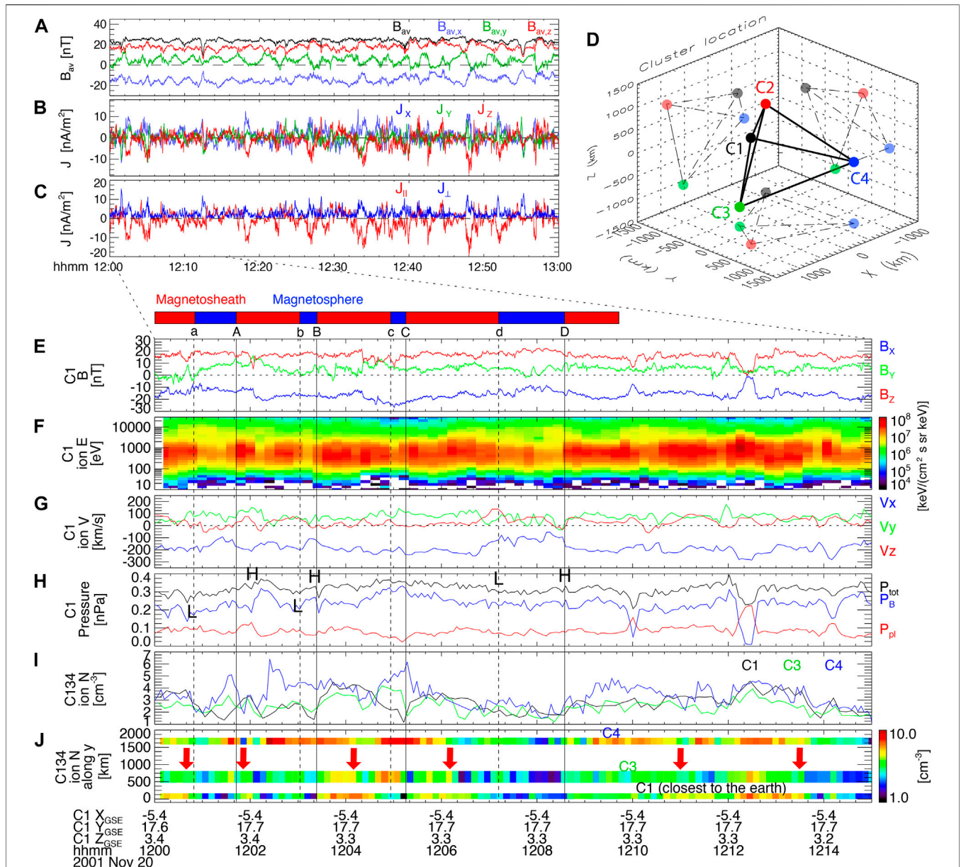
FIGURE 1 | Cluster observation of duskward KHVs: (A) the magnetic field and (B,C) the electric current density during 1,200–1300 UT on 20 November 2001; (D) the tetrahedral configuration of the four Cluster spacecraft around its barycenter at \sim(-5.3, 17.9, 3.2) R_E in GSE. C1 observation from 1200 UT to 1215 UT on 20 November 2001: (E) the magnetic field; (F) the ion energy spectrogram; (G) the ion velocity; (H) the plasma (red) and magnetic (blue) pressures, and the sum (black) of these pressures; (I) the ion density measured by C1 (black), C3 (green), and C4 (blue); (J) the ion density (color) at C1, C3, and C4 arranged in terms of their distance away from the magnetopause (along y; e.g., C1 located closest to the earth).
