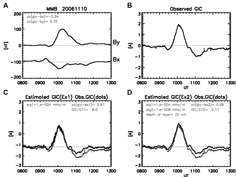
FIGURE 8 | (A, B) B_x , B_y and GIC observed at MMB in the evening (10 UT, 19 MLT) during the substorm bay event. (C) GIC estimated from E_{x1} scaled to the GIC with the scale factor, k_1 = 8.0 [A/(mV/m)] (solid line) and observed GIC (dotted line). (D) GIC estimated from E_{x2} scaled to the GIC with the scale factor, k_2 = 0.17 [A/(mV/m)] (solid line) and observed GIC (dotted line).
