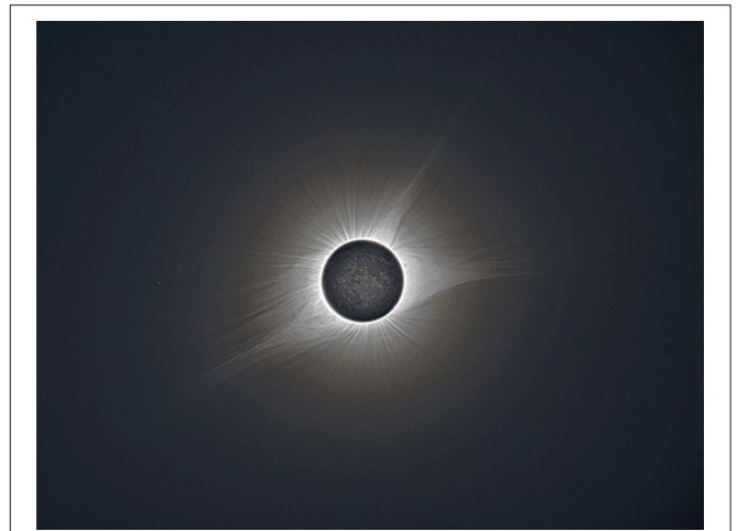
FIGURE 1 | High-contrast imaging showing the paucity of equatorial coronal streamers at this solar-minimum phase of the sunspot cycle, incorporating 11 individual images taken with a Nikon D-810 DSLR camera and a 800-mm Nikkor lens and processed by Christian Lockwood.
