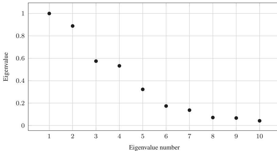
FIGURE 4 | First 10 eigenvalues of A using Gaussian weights and scaling parameter \sigma = 90 for Figure 5A .
