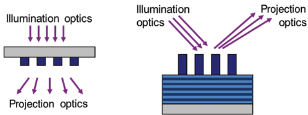
Figure 2: Schematic sketch of transmissive mask for DUV lithography (left) and reflective mask for EUV lithography (right). The multilayer of the EUV mask is only schematically shown. A real Mo/Si multilayer mask blank consists of about 40 bilayers of molybdenum and silicon.
