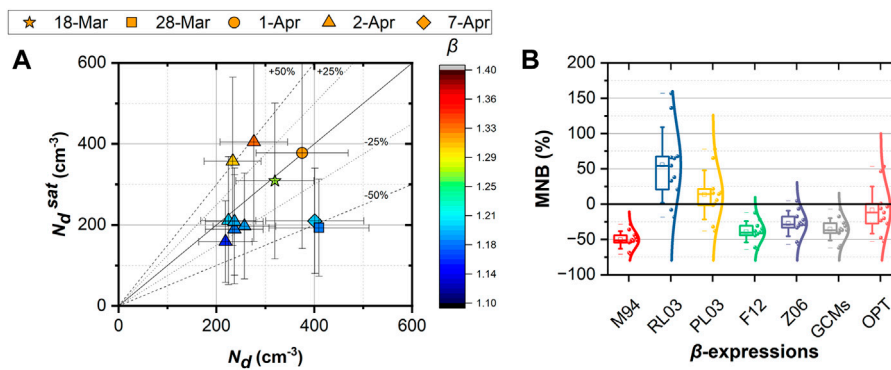
FIGURE 4 (A) Droplet number closure between N_d and N_d^{sat} using the OPT compared to N_d in respect of \beta_{opt} on the colorscale; (B) The MNB of the closure of N_d^{sat} - N_d by using each \beta -expression: (i) M94, ii) RL03, iii) PL03, iv) F12, v) Z06, vi) GCMs, and vii) OPT, respectively.
