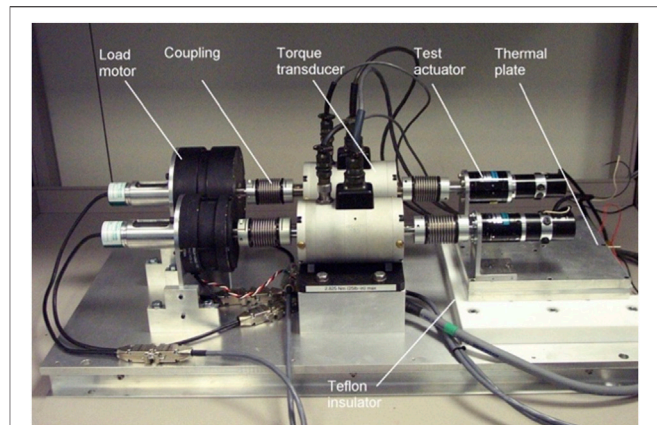
FIGURE 5 | Testing the joints of a space manipulator on a dynamometer using actively controlled loads (CSA).
