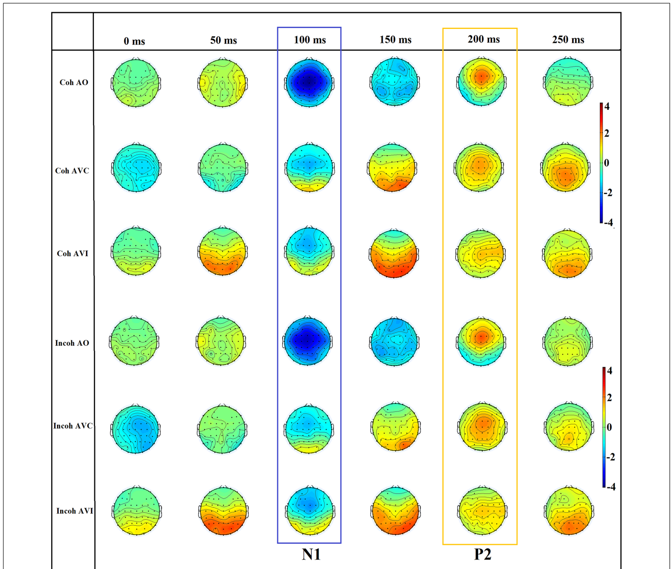
FIGURE 5 | The scalp topography of N1 and P2 for the six conditions (Coh AO, Coh AVC, Coh AVI, Incoh AO, Incoh AVC, Incoh AVI) in time steps of 50 ms. The range of the voltage maps is from -4 to 4 \mu V.
