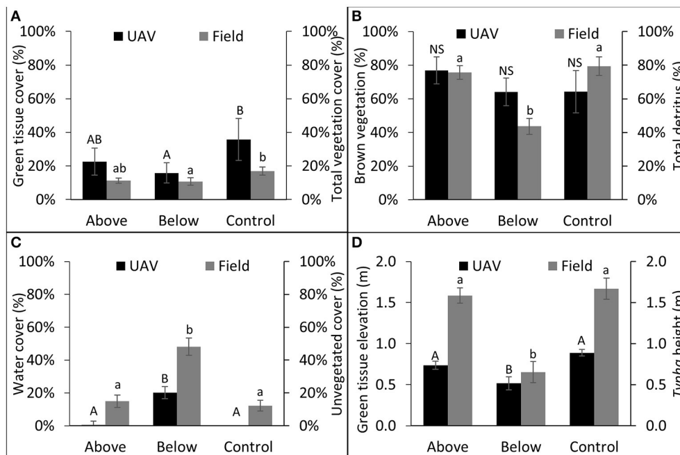
FIGURE 4 | Comparison between UAV collected data and field collected data; UAV variable on left axes and comparable field collected data on right axes. Letter differences denote significant treatment contrasts, UAV data represented by capital letters, field data represented by lowercase letters. NS denotes no significant differences between treatments ( P > 0.05 ). (A) UAV green tissue cover (%) (area with NDVI value > 0.28 /total area); (B) UAV brown tissue cover (%) (area with NDVI values between 0.0 and 0.28/total area); (C) UAV water cover (%) (area with NDVI value > 0.0 /total area); (D) green tissue height (corrected using water average water elevation).
