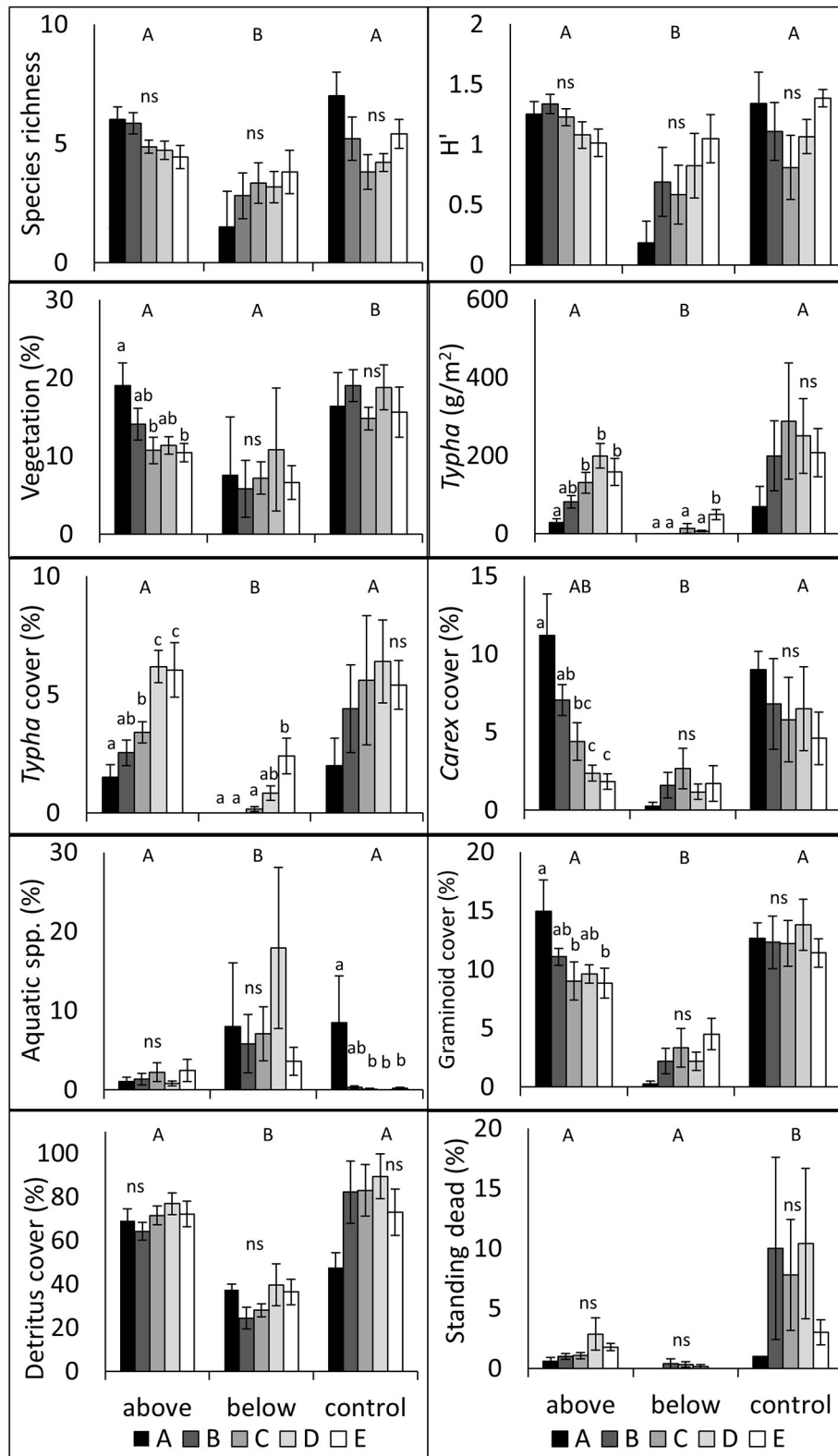
FIGURE 3 | Vegetation responses by treatment and subplot \pm SE in 2016, 1-year following treatment implementation. Capital letters denote significant treatment contrasts; lowercase letters denote within treatment subplot contrasts; ns denotes no significant differences ( P > 0.05 ) between subplots. Subplots approach the center of each stand with alphabetically increasing enumeration.
