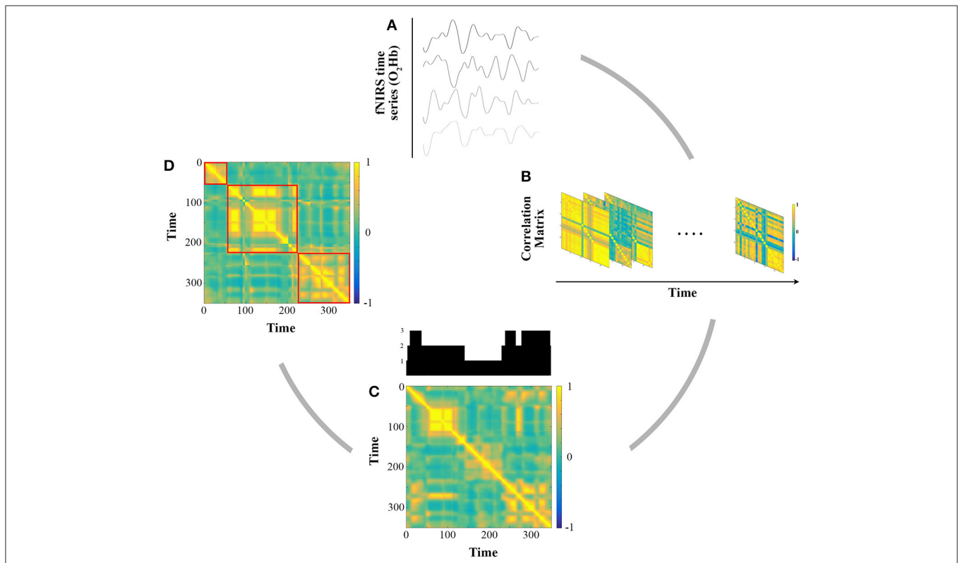
FIGURE 3 | Illustration of the functional connectivity analysis for one representative subject. (A) Extraction of O_2Hb fNIRS time series for all channels after preprocessing and band pass filtering (cut off frequency [0.08 0.009]). (B) Sliding window Pearson's correlation analysis for window sizes of 30, 75, and 120 s. (C) Grand average correlation analysis between each matrix. The upper plot shows communities detected for 360 s (3 communities in this example). (D) Grand average matrix after putting in the order of community. Red squares delimit each community.
