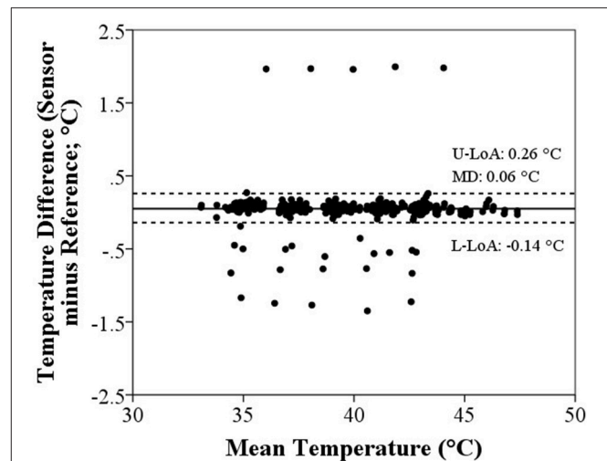
FIGURE 1 | Bland-Altman plot of the agreement between ingestible sensor and reference temperatures. Solid and dashed lines represent the mean difference (MD) and limits agreement (LoA; upper-U, and lower-L), respectively.
