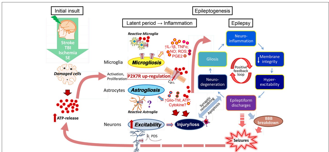
FIGURE 1 | ATP-driven P2X7 activation as possible contributor to epileptogenesis and epilepsy. Brain inflammation has been suggested as a crucial etiopathogenic mechanism of epilepsy contributing to seizure generation and the development of epilepsy (Vezzani et al., 2016). Brain injury (stroke, trauma, ischemia)-induced cell damage and/or cell death associated with an up-regulation of P2X7 on microglia and possibly neurons, leads to a massive release of ATP which then acts as a danger signal resulting in the activation of astrocytes and microglia. The P2X7 in particular has been described as a major regulator of the synthesis and secretion of cytokines (IL-1 \beta , TNF \alpha ) and other inflammatory mediators (NO, ROS, PGE2) via microglial cells. However, the P2X7 may also trigger the release of gliotransmitters (Glio-TM) and ATP from astrocytes and neuronal terminals. Continuing brain inflammation is characterized by astro- and microgliosis with enhanced release of ATP and pro-inflammatory mediators/molecules causing changes in neuronal membrane integrity, modifications of ion channels and consequently neuronal hyperexcitability. This will lead to increased brain susceptibility to seizures initiated by paroxysmal depolarization shifts (PDS), rhythmic burst firing, and epileptiform discharges finally producing focal or generalized seizures. Recurrent seizures per se promote the release of ATP and pro-inflammatory cytokines and activate immune response that sustains seizure recurrence leading to a vicious cycle of increased inflammation and hyperexcitability. Other pathological mechanism may be involved in epileptogenesis and seizure initiation, such as injury and/or loss of neurons, synaptic remodeling (mossy fiber sprouting), BBB breakdown, and lymphocyte accumulation.
