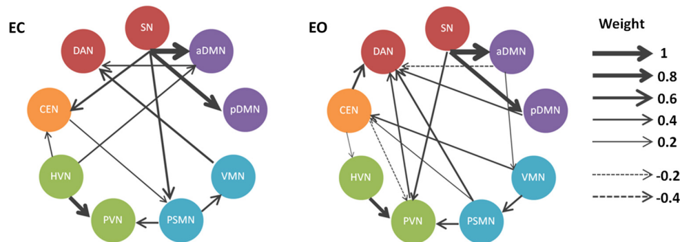
FIGURE 3 | Directional connectivity patterns related to the EO and EC states in the BN model. The RSNs (sphere radius = 6 mm) are graphically connected to depict their conditional dependencies in a BN model. Only
