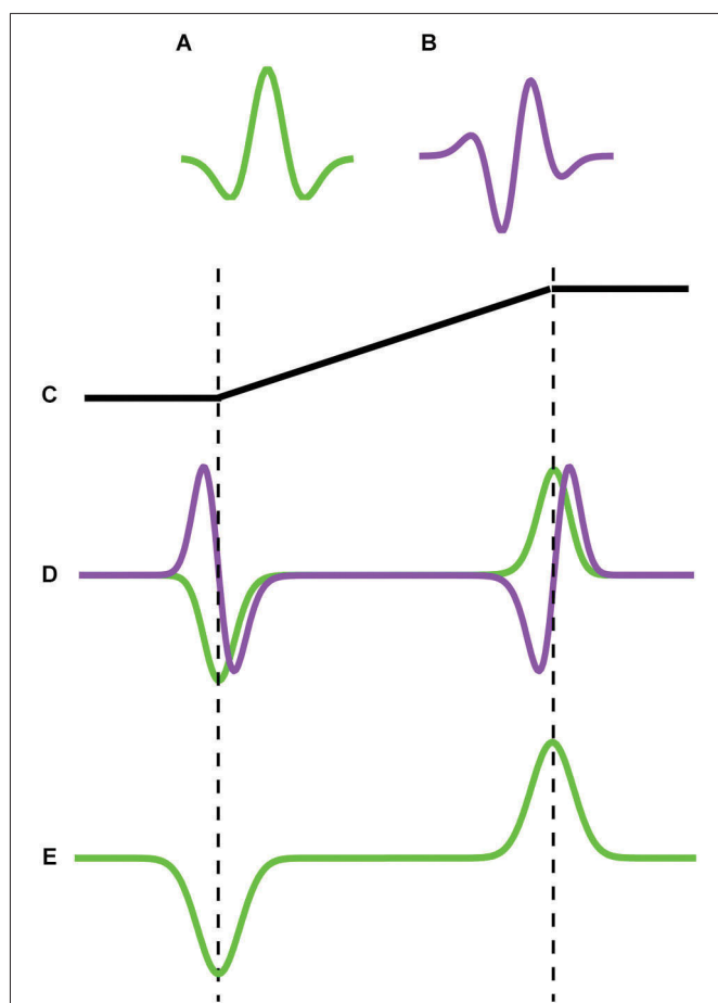
FIGURE 2 | Schematic of the principle behind Feature models of Mach bands that employ even- and odd-symmetric filters. (A) even-symmetric filter. (B) odd-symmetric filter. (C) trapezoidal edge profile. (D) response of even (green) and odd (purple) filters. The even-symmetric filter gives a strong response at the foot and knee of the trapezoid whereas the odd-symmetric filter gives zero response. (E) bars are signaled at the trapezoid's foot and knee.
