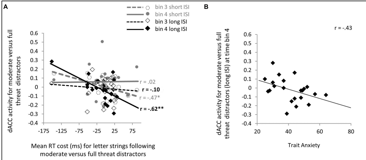
FIGURE 3 | Dorsal ACC (dACC) activity to moderate versus strong threat distractors: relationship with speed of letter target identification (A) and trait anxiety (B). (A) A finite impulse response (FIR) model was used to extract dACC activity from time bins 3 and 4 (4–6 and 6–8 s, respectively) post distractor presentation. For short distractor-target ISI trials, time bin 3 activity may reflect neuronal activity at a time just prior to, through to concurrent with, letter string onset; whereas for long distractor-target ISIs, this is more likely to be captured by time bin 4 activity. In line with this, on short distractor-target ISI trials, greater time bin 3 dACC activity was significantly associated with faster letter target identification following moderate versus
