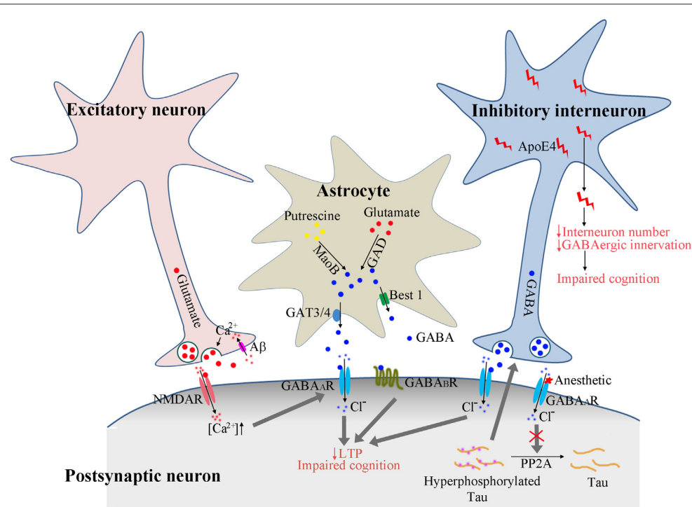
FIGURE 1 | Proposed model of GABAergic signaling in AD pathogenesis. Calcium enters the presynaptic terminal via A \beta formed pores on cell membrane. The increased calcium concentration triggers presynaptic glutamate neurotransmitter release and activates postsynaptic receptors. The activated NMDA receptors further enhance the GABA A receptor activation to dampen the overexcitation. In astrocytes, GABA could be synthesized from putrescine or glutamate and released via GAT3/4 or Best1 channel. The release of GABA from astrocytes may be enhanced under AD conditions to activate the extrasynaptic GABA A and GABA B receptors, resulting in suppressed long-term potentiation (LTP) and impaired cognition. The activation of GABA A receptors by anesthetics reduces PP2A binding with tau protein, resulting in tau hyperphosphorylation, which feeds back and enhances the activation of GABAergic interneurons and GABA release. ApoE4 secreted from GABAergic interneurons results in reduced interneuron number and reduced GABAergic innervation to other neurons, eventually leading to the disruption of neuronal circuitry and impaired cognition.
