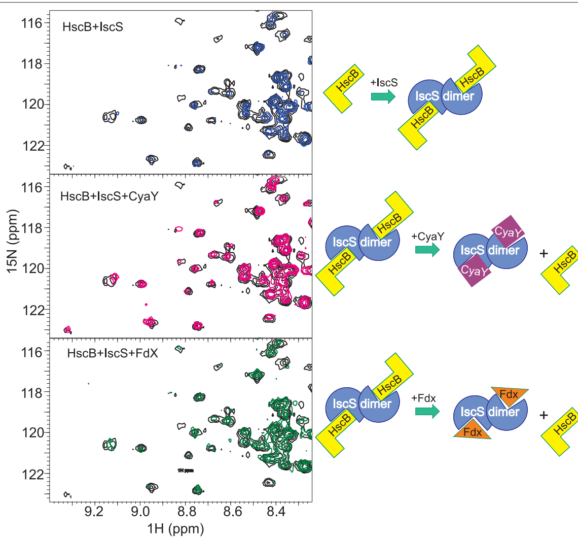
FIGURE 5 | Competition experiments of HscB with CyaY and Fdx. (Top) Superposition of the HSQC spectra of 100 \mu M free ^{15} N-labeled HscB (black) and in the complex with unlabeled IscS 1:1 (blue). (Middle) HSQC spectra of 100 \mu M ^{15} N-labeled HscB in complex with IscS with the addition of CyaY (1:1:3). (Bottom) HSQC spectra of 100 \mu M ^{15} N-labeled HscB in the presence of IscS and apo-Fdx (1:1:3). The experiments are summarized schematically on the right.
