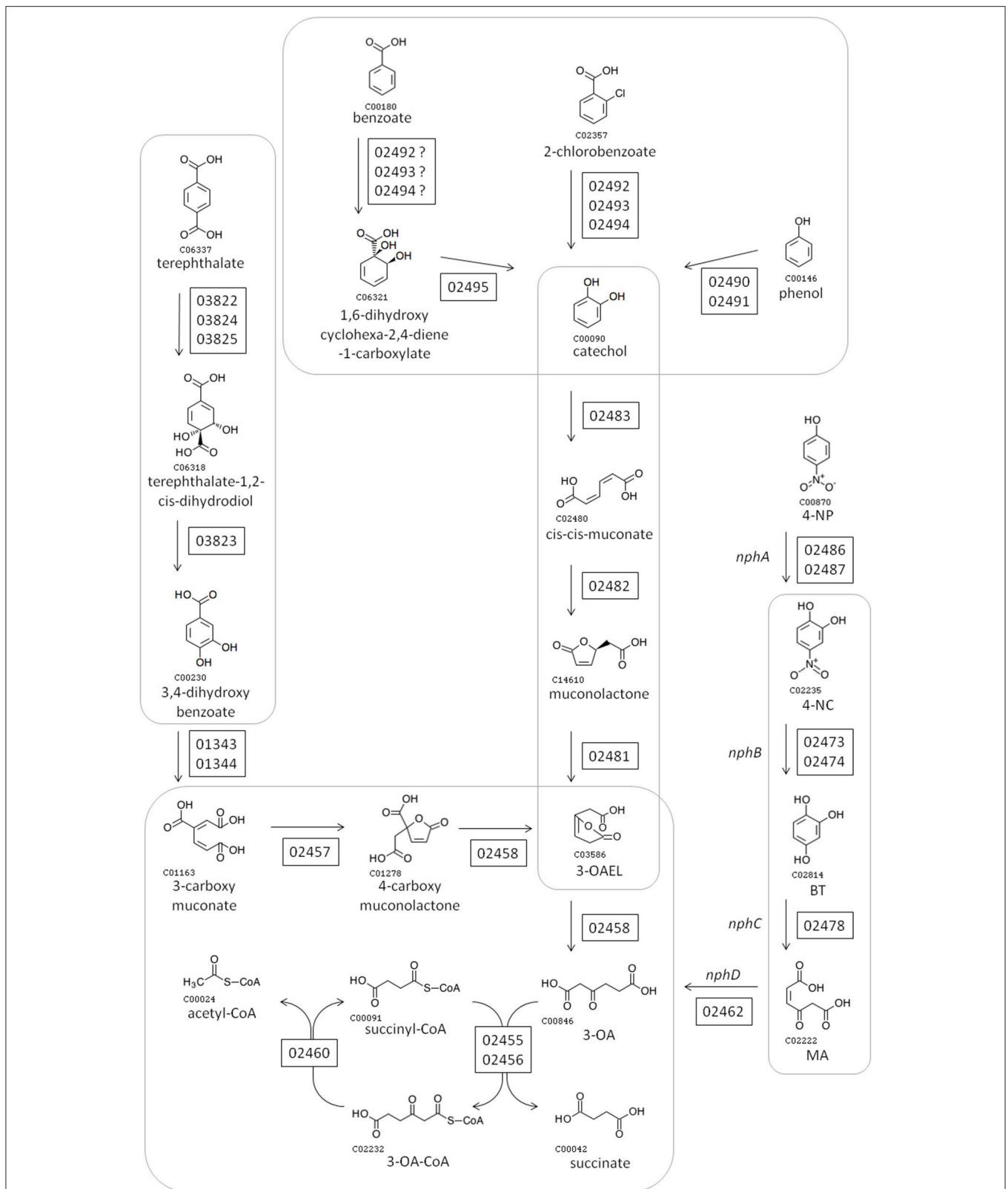
FIGURE 2 | Proposed pathway for degradation of 4-NP and other aromatic compounds by BUPNP1. Numbers in rectangles near enzymatic steps represent BUPNP1 locus tag numbers for the genes encoding the enzyme(s) in question. Enzymatic reactions enclosed together in smooth-cornered rectangles can be considered sub-pathways, with successive conversions catalyzed by enzymes encoded in a putative operon. 3-OA, 3-oxoadipate; 4-NP 4-nitrophenol; 4-NC, 4-nitrocatechol; BT, benzene-1,2,4-triol; MA, maleyl acetate; 3-OAEL, 3-oxoadipate-enol-lactone.
