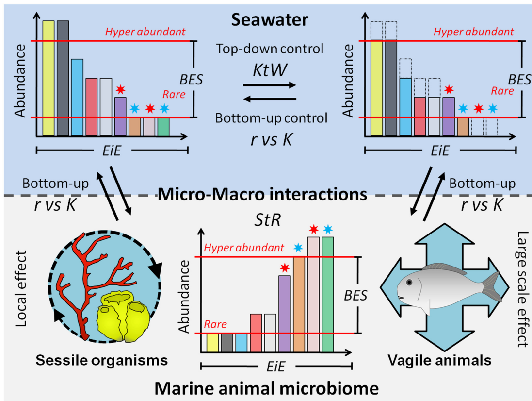
FIGURE 5 | Relation between “sustaining the rare” hypothesis and other classical microbial theories. ST R : Sustaining the Rare, the hypothesis introduced in this paper. E i E: Everything is Everywhere – B E S: But Environment Selects, the two tenets of Baas Becking dictum. K t W: Killing the Winner, top-down control of the more abundant and fast growing microbial population through viral lysis. r vs. K: ecological strategies of microbes influencing their response to bottom-up and top-down factors of control. Asterisks on the abundance distributions represent the two types of host-associated microbes discussed in the main text, symbionts/mutualists (blue) and opportunist copiotrophs (red).
