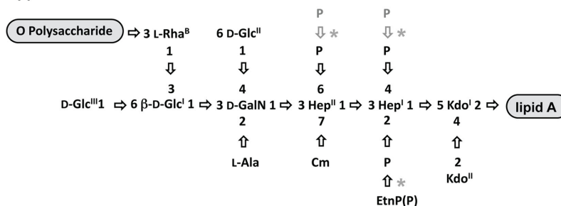
FIGURE 4 | Structures of uncapped and capped glycoforms. The structures of the uncapped core oligosaccharide (A), and capped core oligosaccharide (B) are depicted. All the sugars shown have \alpha configuration unless otherwise indicated. Asterisks depict variable substitutions, acetylation sites are shown since they have not been precisely identified. Ala, alanine; Cm, carbamoyl; Etn, ethanolamine; GalN, 2-amino-2-deoxy-galactose (galactosamine); Glc, glucose; Hep, L-glycero-D-manno-heptose; Kdo, 3-deoxy-D-manno-oct-2-ulosonic acid; Rha, rhamnose. Adapted from King et al. (2009).
