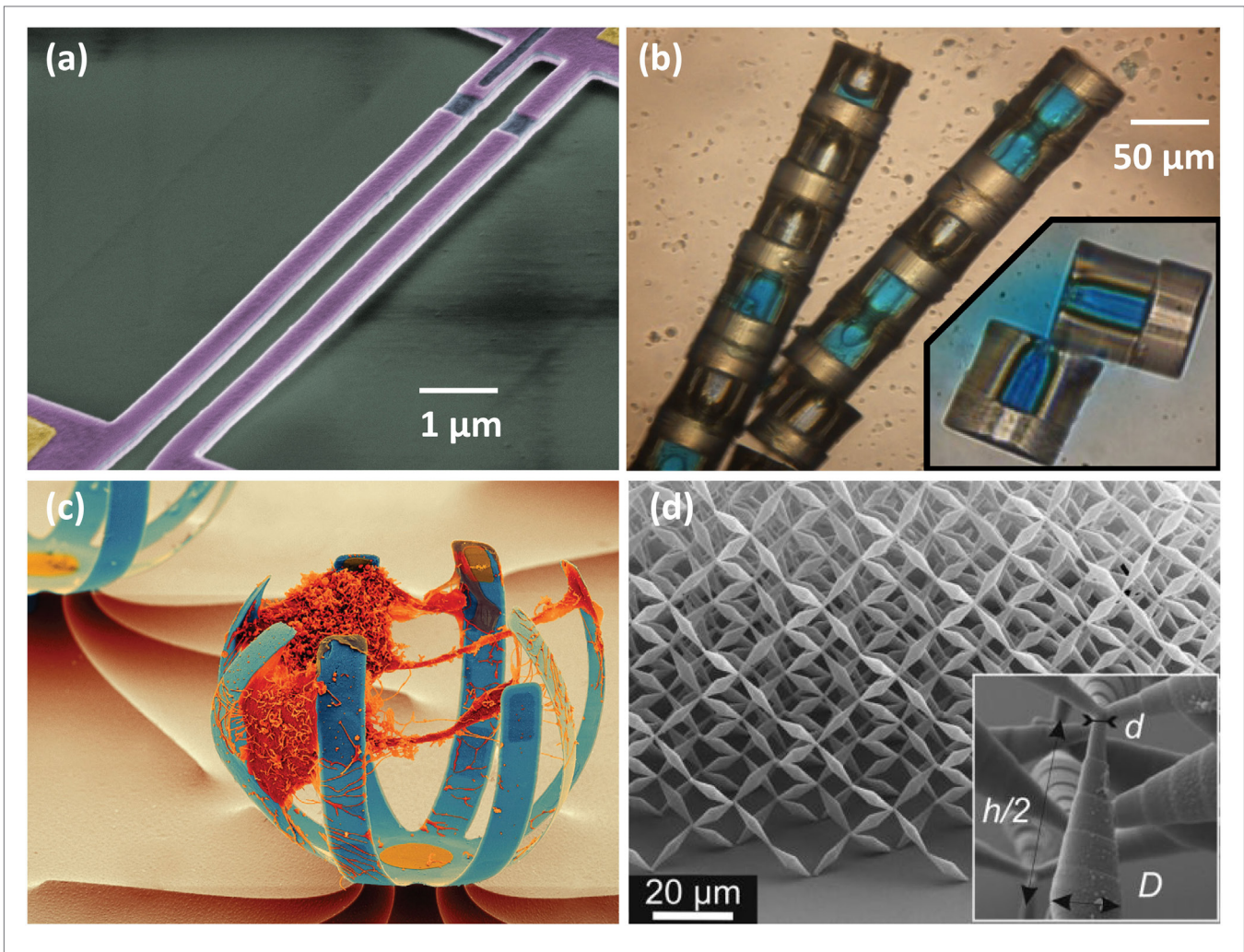
FIGURE 2 | State of the art for micro- and nano-mechanical devices in research. (A) Scanning electron microscope (SEM) micrograph of two NEMS clamped-clamped beams. The beams are mechanically coupled through the ledge present in the anchoring region and they are fabricated using a combination of metal and piezoelectric layers, which provide the devices with self-sensing and actuating capabilities. These devices are used as coupled resonators to study complex dynamics in the nanoscale (Villanueva et al., 2011, 2013) and they also have potential for noise reduction in communications (Kenig et al., 2012) and sensitivity increase for sensing (Spletzer et al., 2006). Color has been artificially added for illustration purposes. (B) Optical microscope picture of an assembly in liquid medium of hollow half-cylinders fabricated in SU-8. Fluidic self-assembly is one of the promising novel ways that can be used to assemble MEMS/NEMS devices in large scale (Goldowsky et al., 2013; Jacot-Descombes et al., 2013). The coupled cylinders shown in the figure could be used, for example, as microcapsules for drug storage and subsequent local drug release. (C) SEM micrograph of sets of metallic cantilevers with an engineered intrinsic stress gradient in order to obtain the curvature of the cantilevers and the cage-like structures. These cages can be used to capture cells and study their behavior as a function of different cage stiffness (Marelli et al., 2014). This example is an illustration of 2.5-D MEMS devices, where shapes and structures are designed to come out of the plane, as opposed to standard planar technology. Color has been artificially added for illustration purposes. Reproduced by permission of The Royal Society of Chemistry. (D) SEM micrograph of a polymer-based mechanical metamaterial fabricated using 3D printing in the nanoscale (Kadic et al., 2012). Metamaterials are artificially fabricated periodic structures that extend over long periods of space in 1, 2, or 3 dimensions that confer the overall extended pattern of special properties that, in most cases, cannot be found in reality. The mostly studied metamaterials are those giving rise to negative optical refractive indexes (these can be used to engineer invisibility cloaks) (Schittny et al., 2015) and those giving rise to negative Poisson's ratios or negative mass-density tensors, for example, to engineer dilatational materials (Kadic et al., 2012). Reprinted with permission from AIP Publishing LLC.
