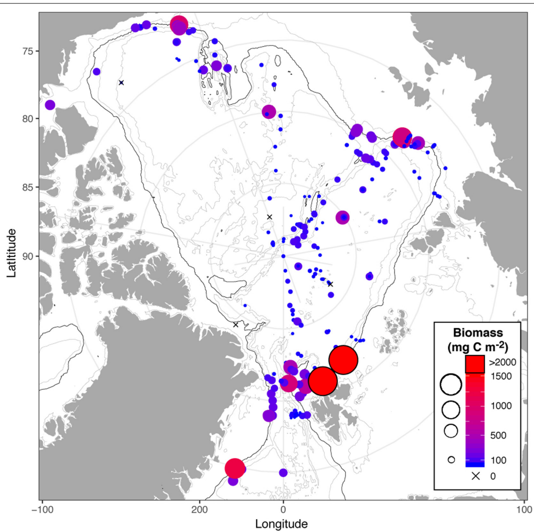
FIGURE 1 | Biomass of benthic macrofauna in the Arctic Ocean basins and adjacent areas (data compiled from Bluhm et al., 2015; Degen et al., 2018; Vedenin et al., 2018). Note biomass values for depths \geq 500 m are included in the figure to show the decline from the upper slope to the central basins. The 1000 m isobaths is depicted as a black line.
