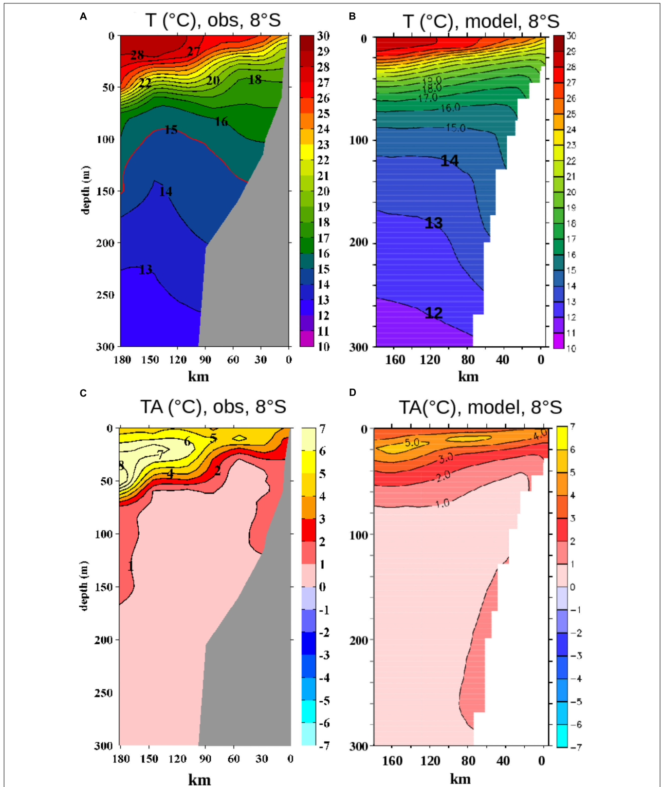
FIGURE 5 | Cross-shore vertical sections of temperature (A,B) absolute values and (C,D) anomalies (in °C) in March 2017 off the northern Peru shelf (Chicama, 8°S). The section’s location is indicated in Figure 4C. Observed anomalies (c) were computed with respect to a climatology of IMARPE data for the period 1981–2010, while modeled anomalies were computed with respect to a model climatology for 2013–2016.
