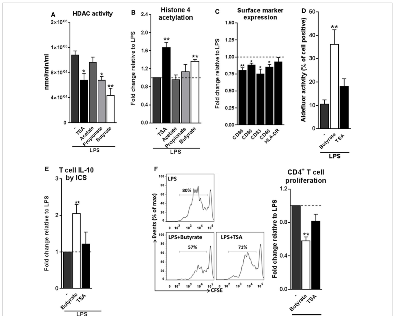
FIGURE 4 | Histone deacetylases (HDAC) inhibition by butyrate is not sufficient for inducing type 1 regulatory T cells-promoting human toIDCs. (A) Dendritic cells (DCs) were stimulated for 24 h with indicated reagents and then assayed for HDAC activity. (B) Analysis of histone 4 acetylation by flow cytometry of DCs stimulated with indicated reagents for 6 h. (C) The expression of maturation markers of DCs stimulated for 48 h with TSA was analyzed using flow cytometry. The expression of surface marker levels is based on the geometric mean fluorescence. (D) Retinaldehyde dehydrogenase activity assay as described in Figure 3D. (E) IL-10 production by T cells as described in Figure 2B. (F) T-cell suppression assay as described in Figure 2D. (A–F) Bar graphs represent means \pm SEM of at least three experiments and (B,C,E,F) are shown as fold change relative to control conditions. * p < 0.05 , ** p < 0.01 , *** p < 0.001 based on paired Student's t -test.
