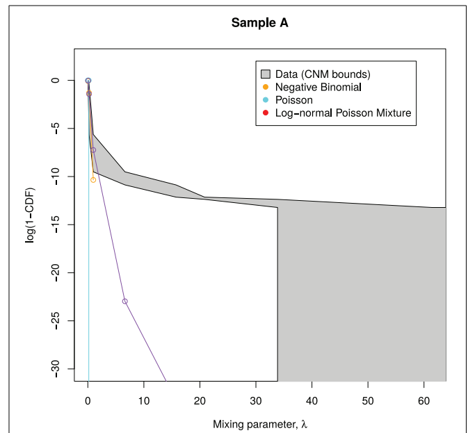
FIGURE 3 | Candidate mixing distributions, and their consistency with the CNM-derived mixing distribution. For clarity, we plot \log(1 - CDF) where CDF is the Cumulative Density Function of \Lambda , and values are calculated only at CNM's \lambda support points. A mixing distribution that is consistent with CNM's predicted mixing distribution, as derived in Section 3.2, would have a line contained within the shaded region, with the black lines representing upper and lower bounds. Here, the lines do not stay within the bounds, indicating that all of the models deviate from CNM's prediction.
