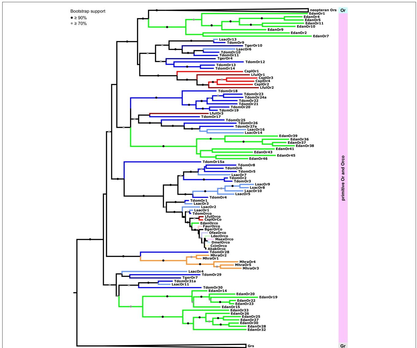
FIGURE 4 | Maximum likelihood tree of Ors focusing on the primitive Or group including Orco within the phylogeny. Enlargement of the maximum likelihood tree shown in Figure 3 . Tree is rooted using Grs as the outgroup. Node support is presented as transfer bootstrap percentages. Different colors represent different species. Different orders are represented by different color hues. Lsac, Lepisma saccharina (light blue); Tger, Tricholepidion gertschi (dark blue); Tdom, Thermobia domestica (blue); Mhra, Machilis hrabei (orange); Edan, Ephemera danica (green); Lful, Ladona fulva (red); Cspl, Calopteryx splendens (dark red); Faur, Forficula auricularia (desaturated red); Ofas, Oncopeltus fasciatus (desaturated purple); Ccin, Cephus cinctus (desaturated yellow); Ldec, Leptinotarsa decemlineata (desaturated green); Msex, Manduca sexta (desaturated pink); Dmel, Drosophila melanogaster (desaturated blue); Bger, Blattella germanica (brown); Abak, Apocrypta bakeri (brown).
